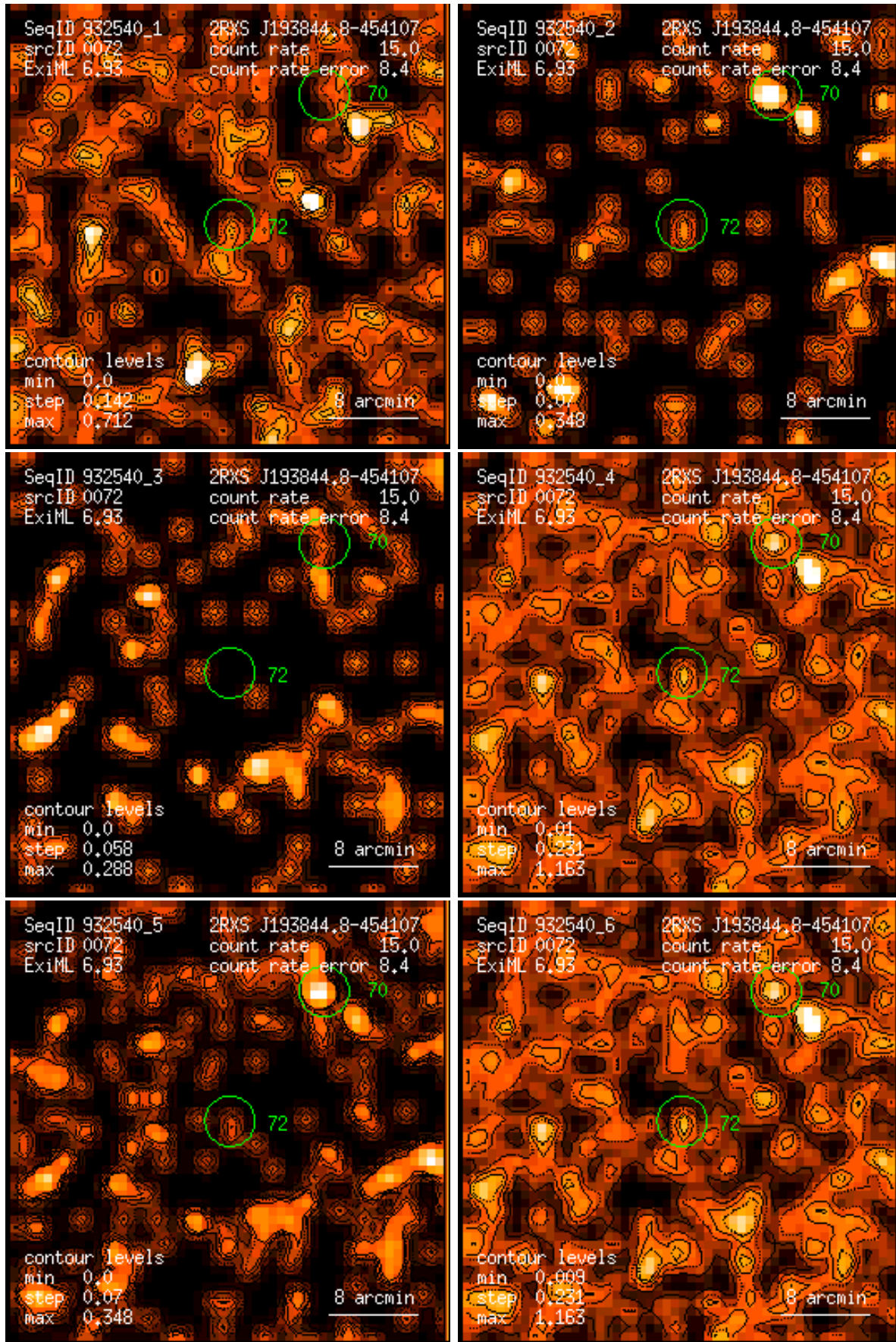
Figure 72: RASS 932540: detection 0072: band rate images, Gaussian filter: (1) PSPC channels 11 – 41, (2) 52 – 90, (3) 91 – 201, (4) 11 – 235, (5) 52 – 201, (6) 11 – 201. Broad band rates in counts/ks. Band rate contour levels in counts/ks/arcmin 2 .
