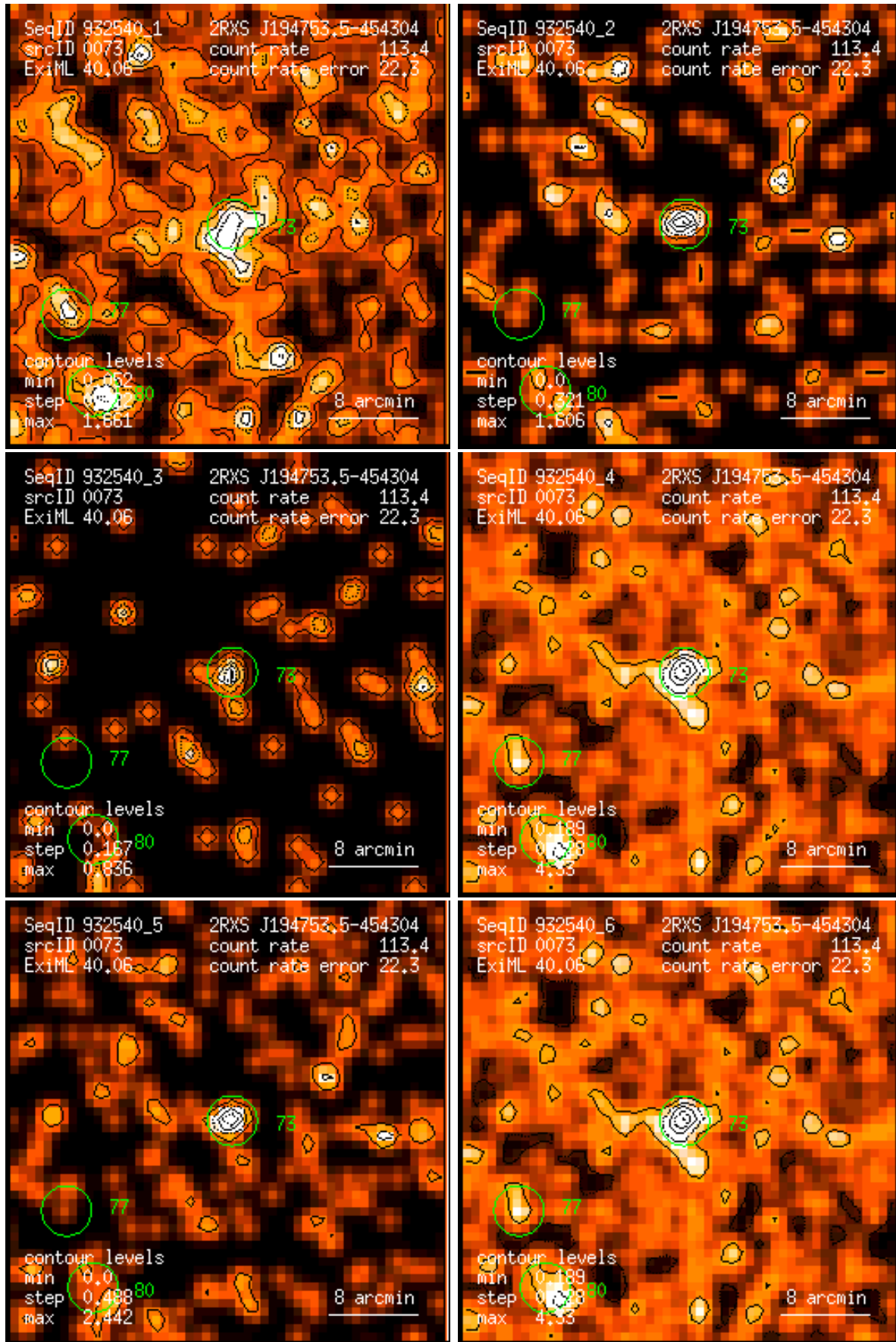
Figure 73: RASS 932540: detection 0073: band rate images, Gaussian filter: (1) PSPC channels 11 – 41, (2) 52 – 90, (3) 91 – 201, (4) 11 – 235, (5) 52 – 201, (6) 11 – 201. Broad band rates in counts/ks. Band rate contour levels in counts/ks/arcmin 2 .
