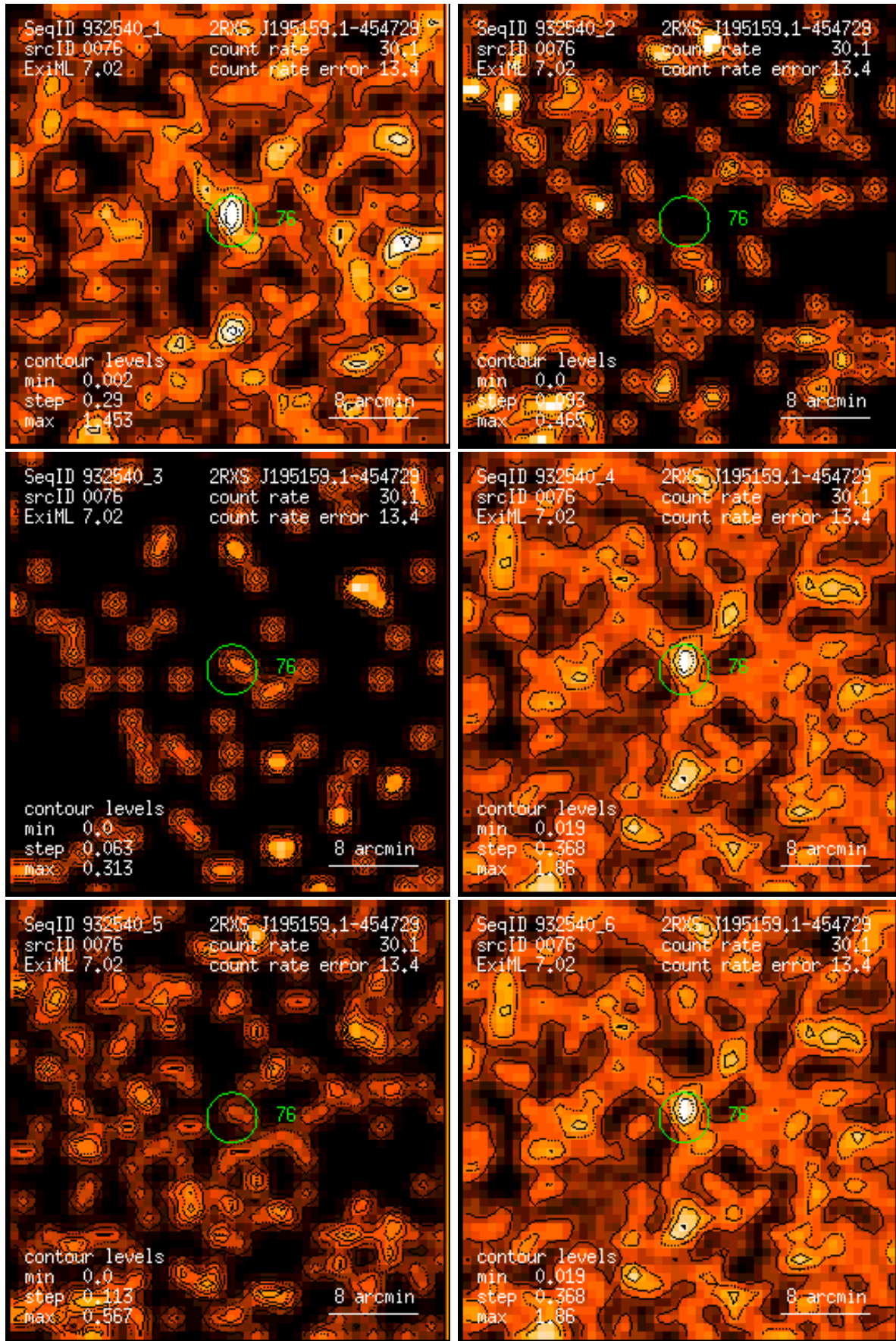
Figure 76: RASS 932540: detection 0076: band rate images, Gaussian filter: (1) PSPC channels 11 – 41, (2) 52 – 90, (3) 91 – 201, (4) 11 – 235, (5) 52 – 201, (6) 11 – 201. Broad band rates in counts/ks. Band rate contour levels in counts/ks/arcmin 2 .
