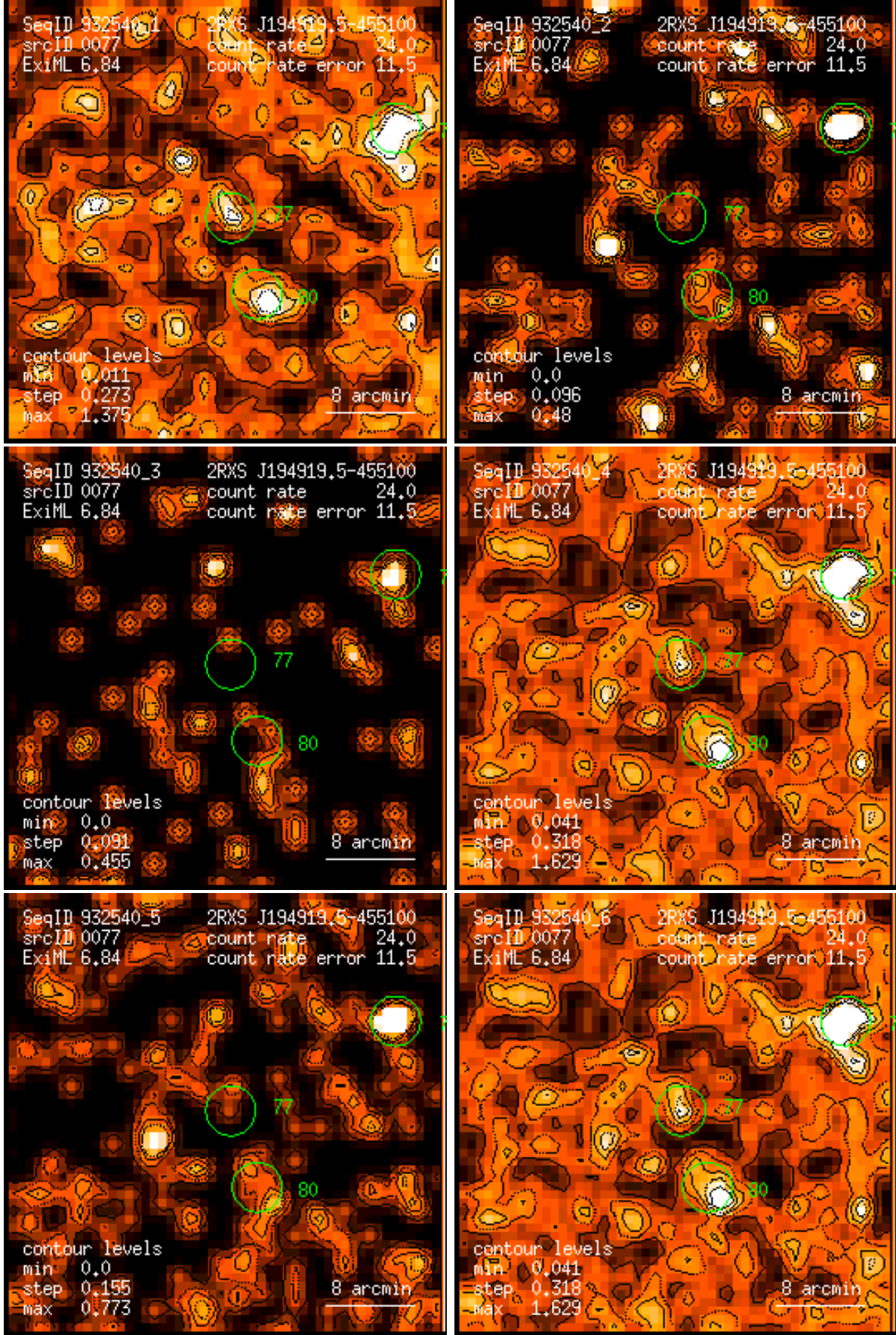
Figure 77: RASS 932540: detection 0077: band rate images, Gaussian filter: (1) PSPC channels 11 – 41, (2) 52 – 90, (3) 91 – 201, (4) 11 – 235, (5) 52 – 201, (6) 11 – 201. Broad band rates in counts/ks. Band rate contour levels in counts/ks/arcmin 2 .
