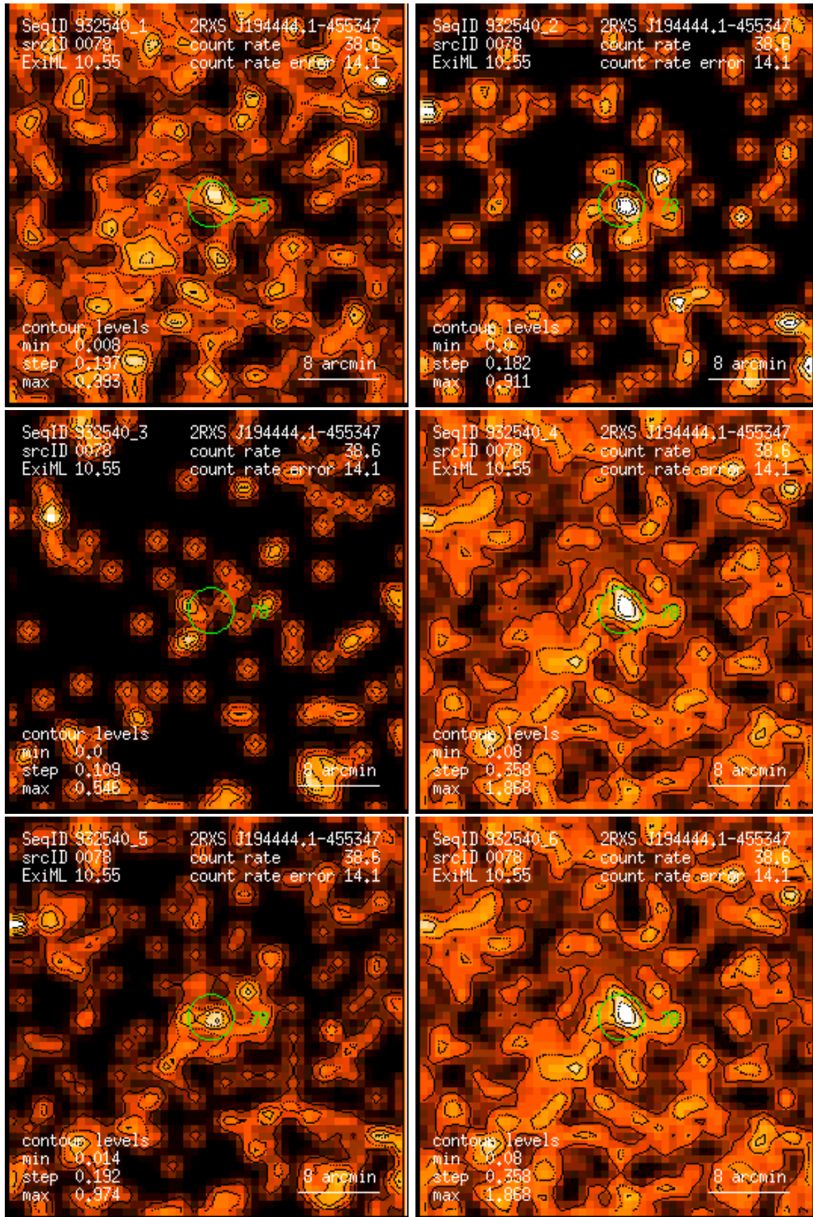
Figure 78: RASS 932540: detection 0078: band rate images, Gaussian filter: (1) PSPC channels 11 – 41, (2) 52 – 90, (3) 91 – 201, (4) 11 – 235, (5) 52 – 201, (6) 11 – 201. Broad band rates in counts/ks. Band rate contour levels in counts/ks/arcmin 2 .
