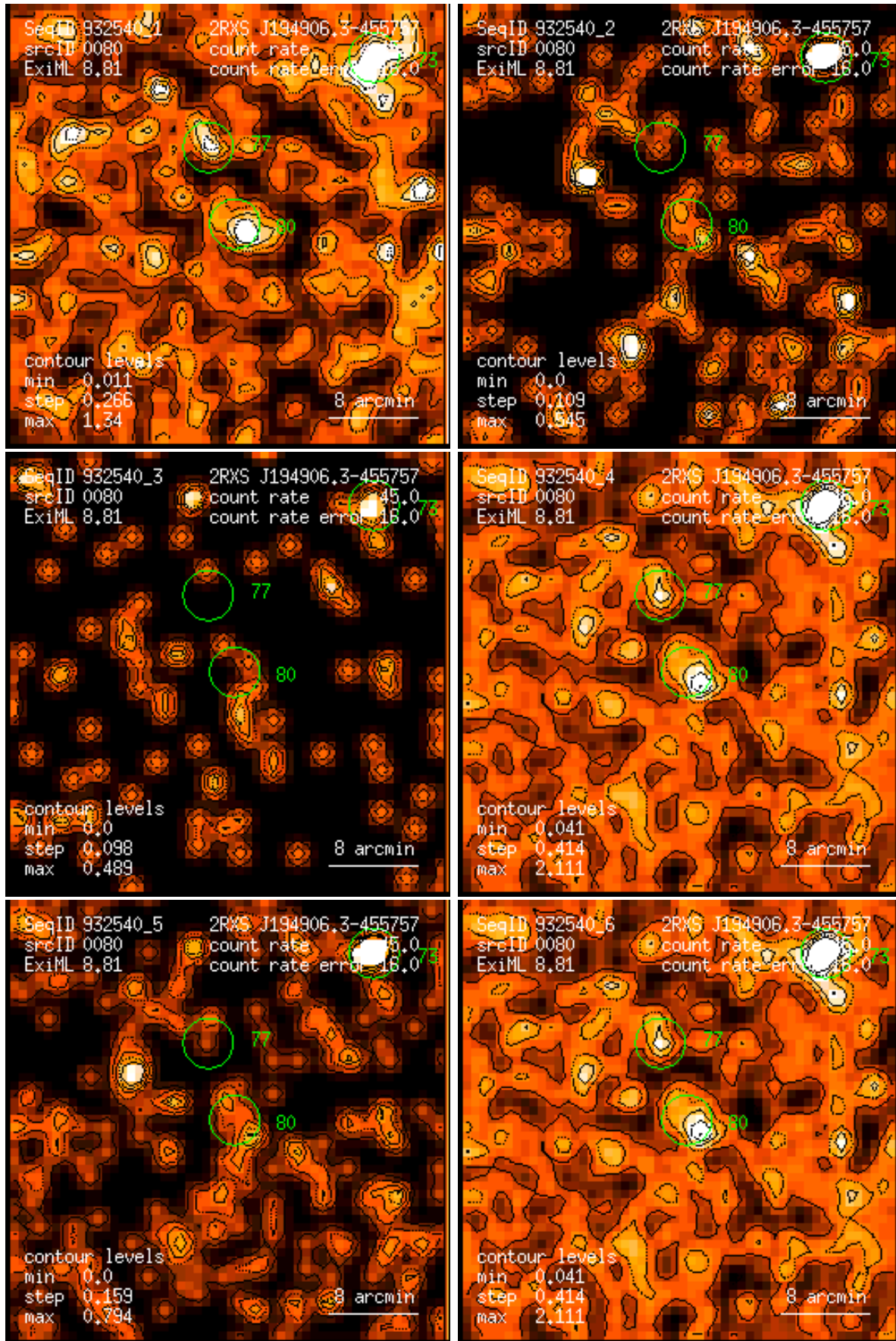
Figure 80: RASS 932540: detection 0080: band rate images, Gaussian filter: (1) PSPC channels 11 – 41, (2) 52 – 90, (3) 91 – 201, (4) 11 – 235, (5) 52 – 201, (6) 11 – 201. Broad band rates in counts/ks. Band rate contour levels in counts/ks/arcmin 2 .
