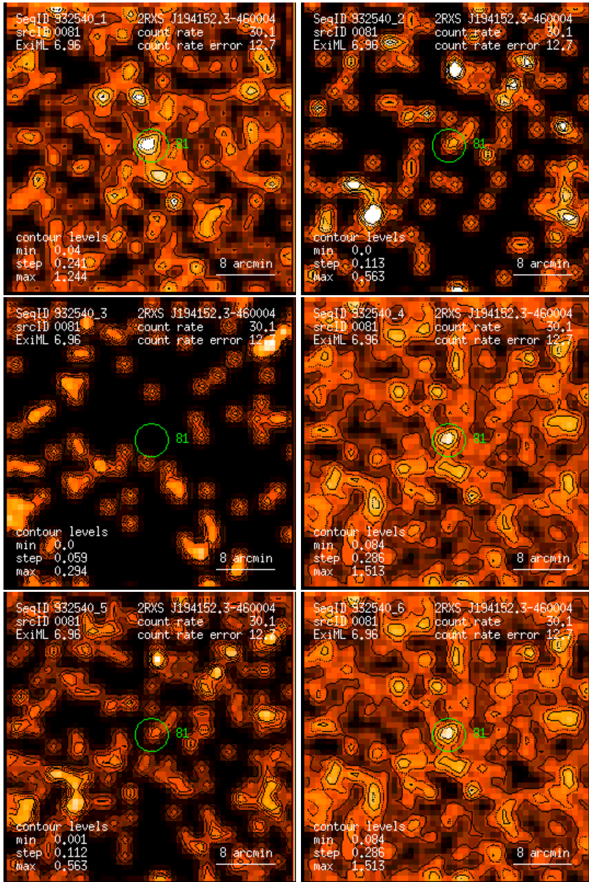
Figure 81: RASS 932540: detection 0081: band rate images, Gaussian filter: (1) PSPC channels 11 – 41, (2) 52 – 90, (3) 91 – 201, (4) 11 – 235, (5) 52 – 201, (6) 11 – 201. Broad band rates in counts/ks. Band rate contour levels in counts/ks/arcmin 2 .
