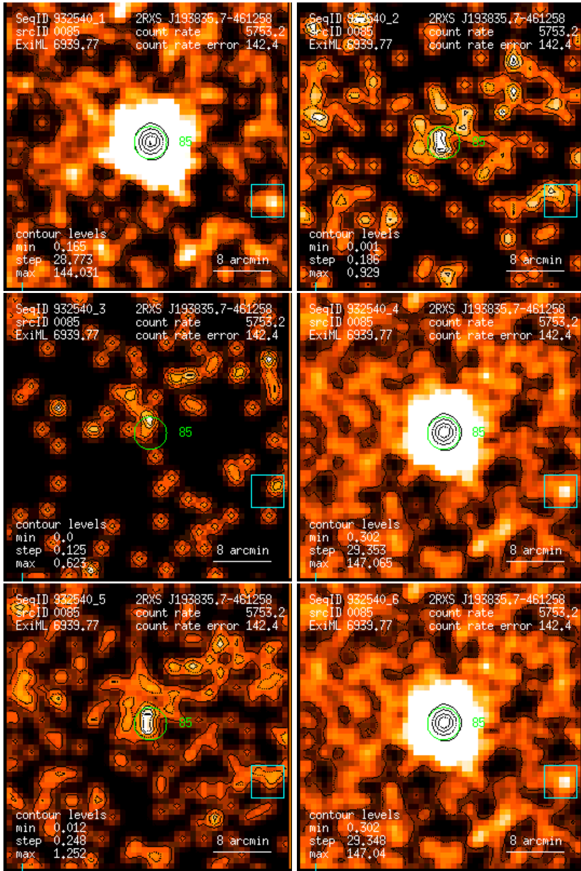
Figure 85: RASS 932540: detection 0085: band rate images, Gaussian filter: (1) PSPC channels 11 – 41, (2) 52 – 90, (3) 91 – 201, (4) 11 – 235, (5) 52 – 201, (6) 11 – 201. Broad band rates in counts/ks. Band rate contour levels in counts/ks/arcmin 2 .
