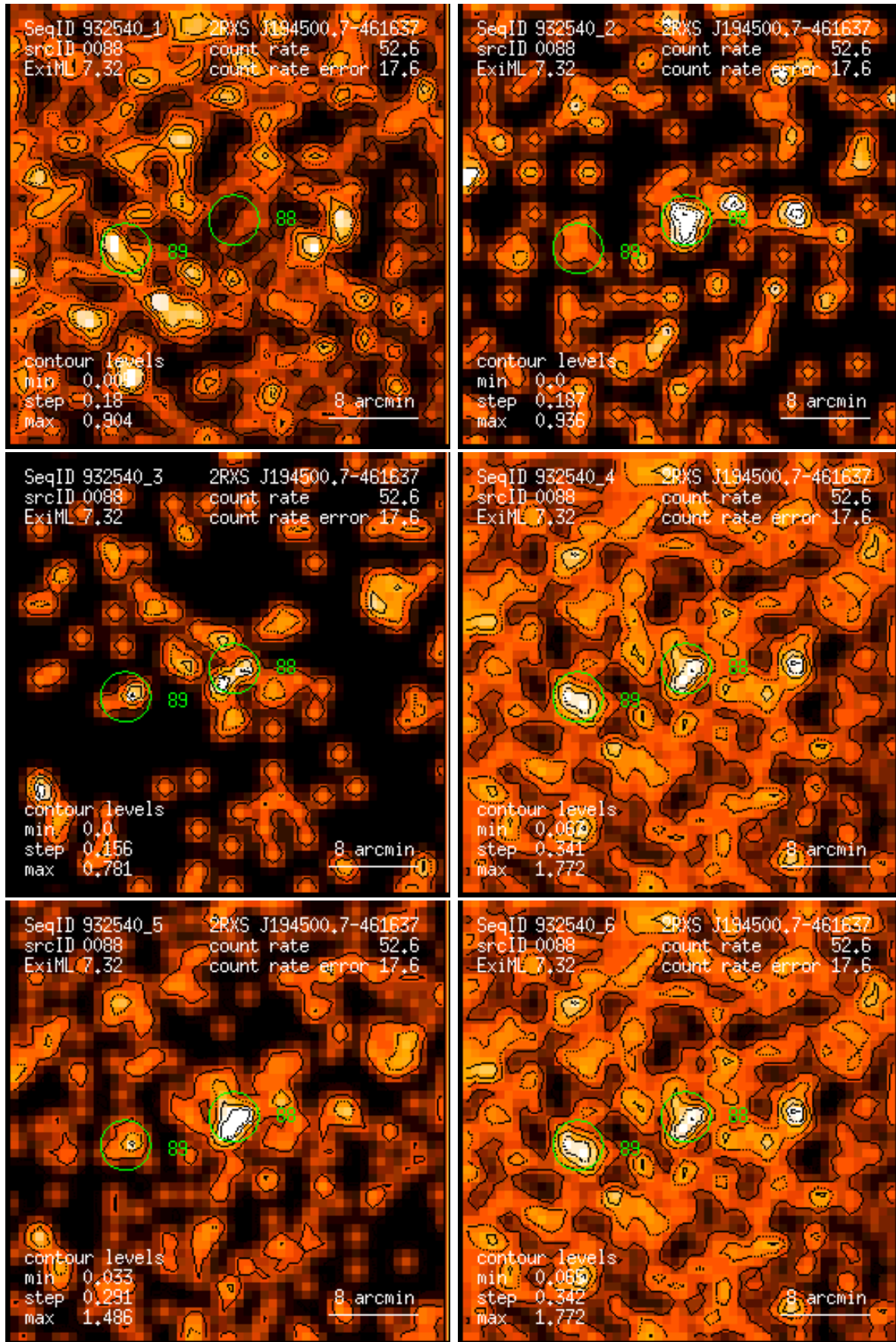
Figure 88: RASS 932540: detection 0088: band rate images, Gaussian filter: (1) PSPC channels 11 – 41, (2) 52 – 90, (3) 91 – 201, (4) 11 – 235, (5) 52 – 201, (6) 11 – 201. Broad band rates in counts/ks. Band rate contour levels in counts/ks/arcmin 2 .
