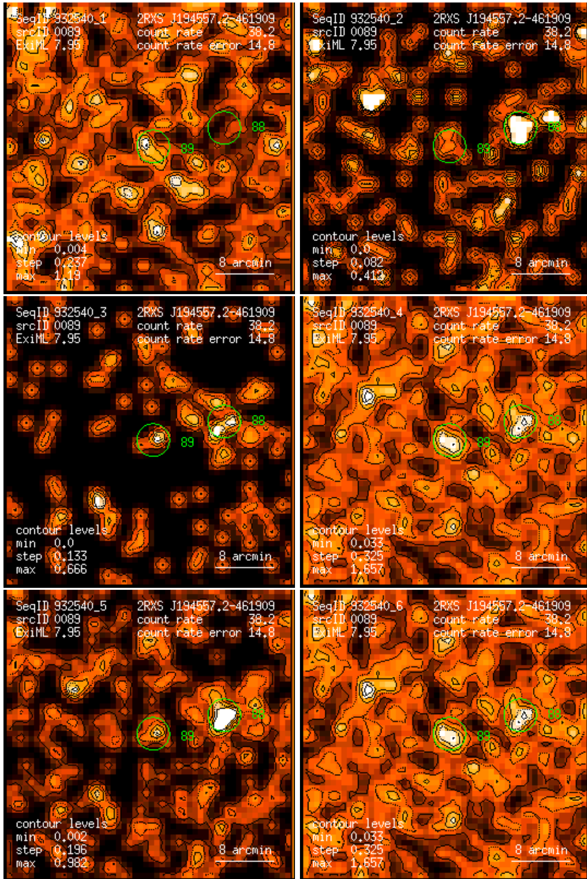
Figure 89: RASS 932540: detection 0089: band rate images, Gaussian filter: (1) PSPC channels 11 – 41, (2) 52 – 90, (3) 91 – 201, (4) 11 – 235, (5) 52 – 201, (6) 11 – 201. Broad band rates in counts/ks. Band rate contour levels in counts/ks/arcmin 2 .
