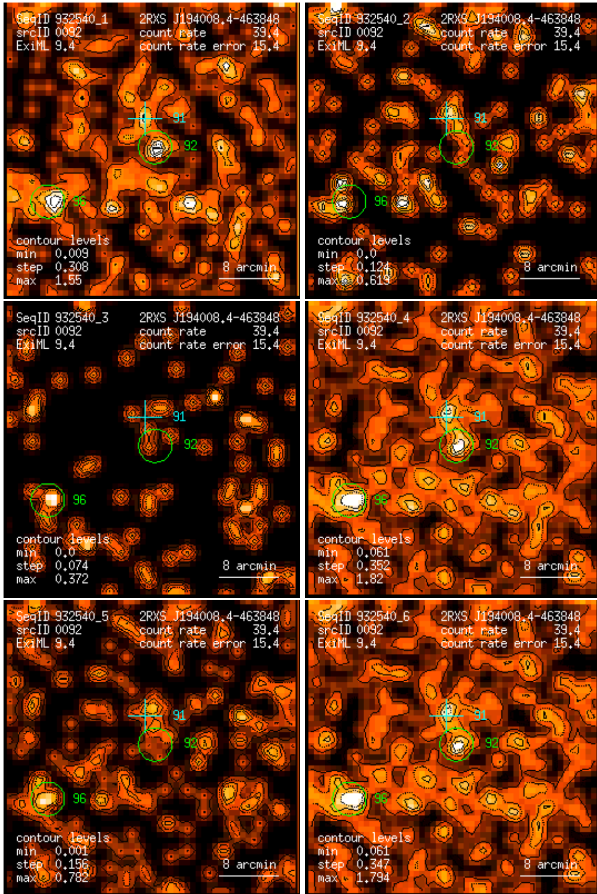
Figure 92: RASS 932540: detection 0092: band rate images, Gaussian filter: (1) PSPC channels 11 – 41, (2) 52 – 90, (3) 91 – 201, (4) 11 – 235, (5) 52 – 201, (6) 11 – 201. Broad band rates in counts/ks. Band rate contour levels in counts/ks/arcmin 2 .
