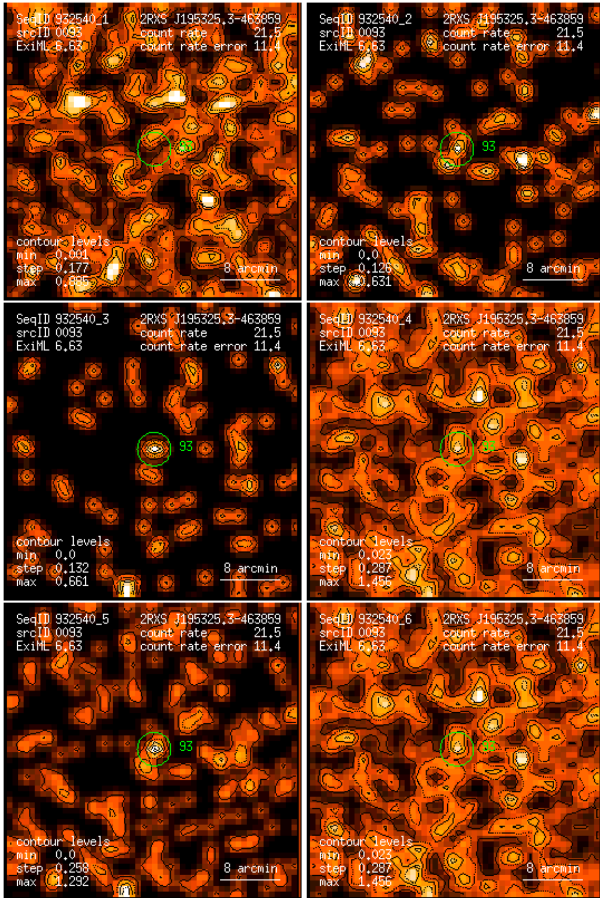
Figure 93: RASS 932540: detection 0093: band rate images, Gaussian filter: (1) PSPC channels 11 – 41, (2) 52 – 90, (3) 91 – 201, (4) 11 – 235, (5) 52 – 201, (6) 11 – 201. Broad band rates in counts/ks. Band rate contour levels in counts/ks/arcmin 2 .
