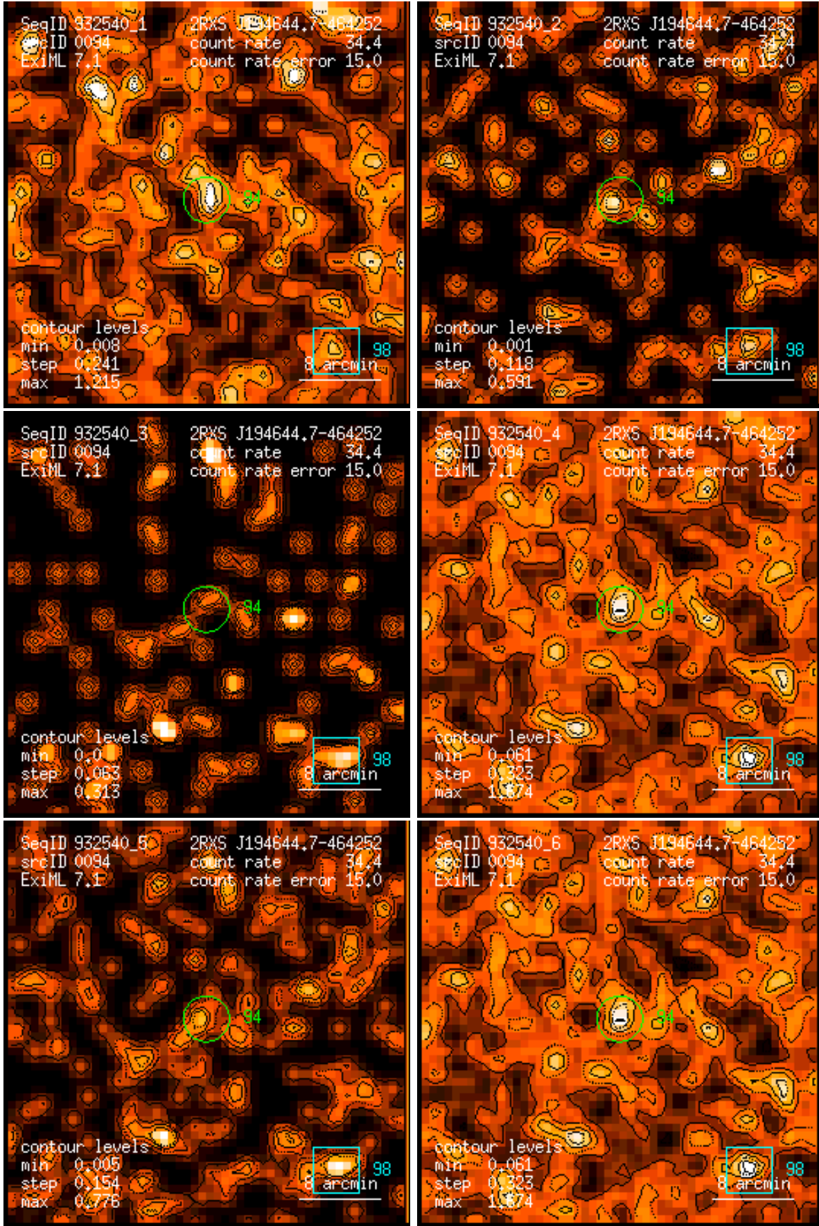
Figure 94: RASS 932540: detection 0094: band rate images, Gaussian filter: (1) PSPC channels 11 – 41, (2) 52 – 90, (3) 91 – 201, (4) 11 – 235, (5) 52 – 201, (6) 11 – 201. Broad band rates in counts/ks. Band rate contour levels in counts/ks/arcmin 2 .
