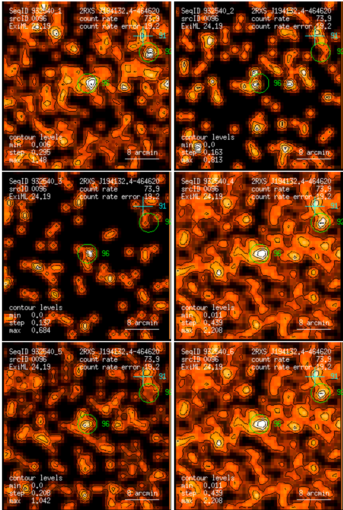
Figure 96: RASS 932540: detection 0096: band rate images, Gaussian filter: (1) PSPC channels 11 – 41, (2) 52 – 90, (3) 91 – 201, (4) 11 – 235, (5) 52 – 201, (6) 11 – 201. Broad band rates in counts/ks. Band rate contour levels in counts/ks/arcmin 2 .
