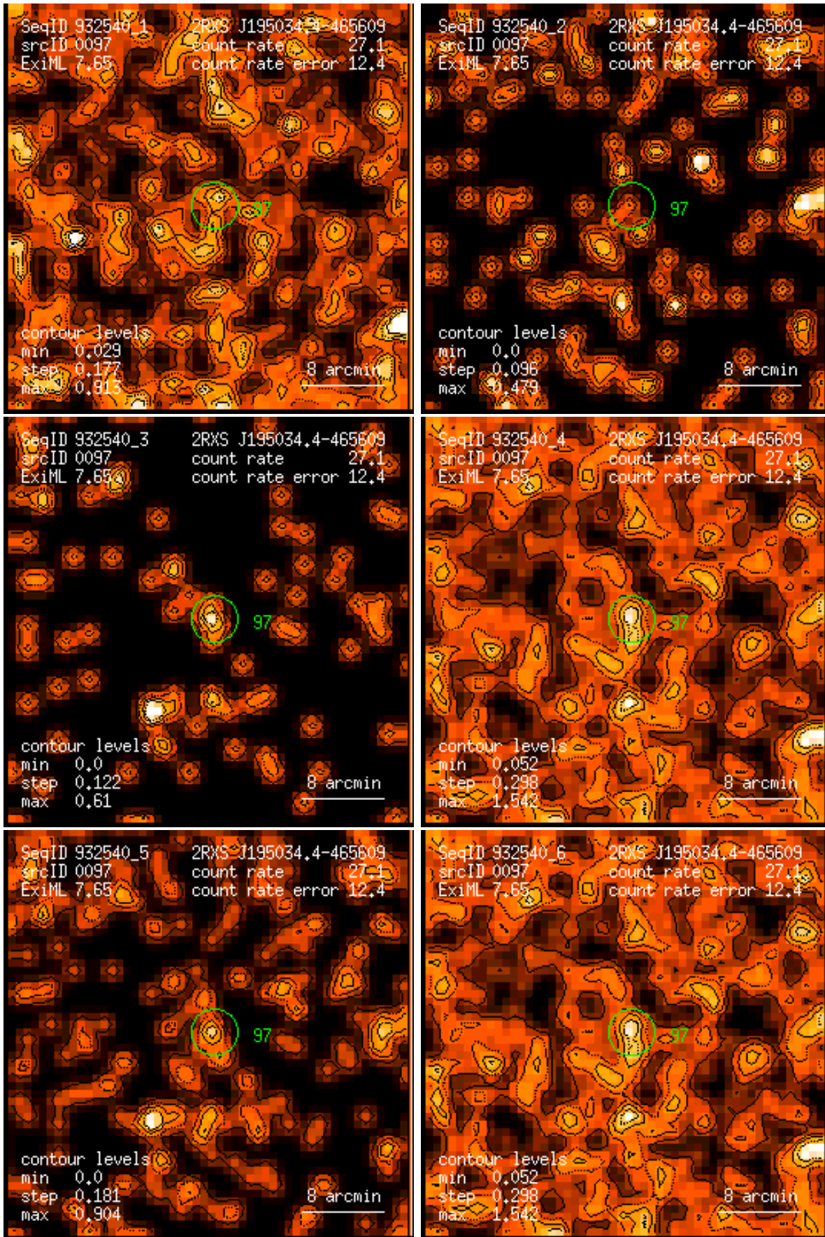
Figure 97: RASS 932540: detection 0097: band rate images, Gaussian filter: (1) PSPC channels 11 – 41, (2) 52 – 90, (3) 91 – 201, (4) 11 – 235, (5) 52 – 201, (6) 11 – 201. Broad band rates in counts/ks. Band rate contour levels in counts/ks/arcmin 2 .
