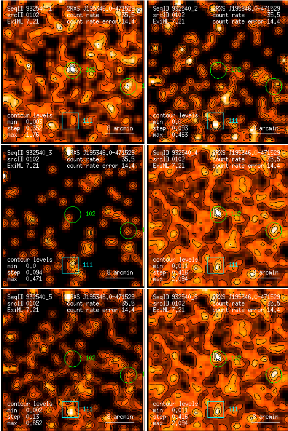
Figure 102: RASS 932540: detection 0102: band rate images, Gaussian filter: (1) PSPC channels 11 – 41, (2) 52 – 90, (3) 91 – 201, (4) 11 – 235, (5) 52 – 201, (6) 11 – 201. Broad band rates in counts/ks. Band rate contour levels in counts/ks/arcmin 2 .
