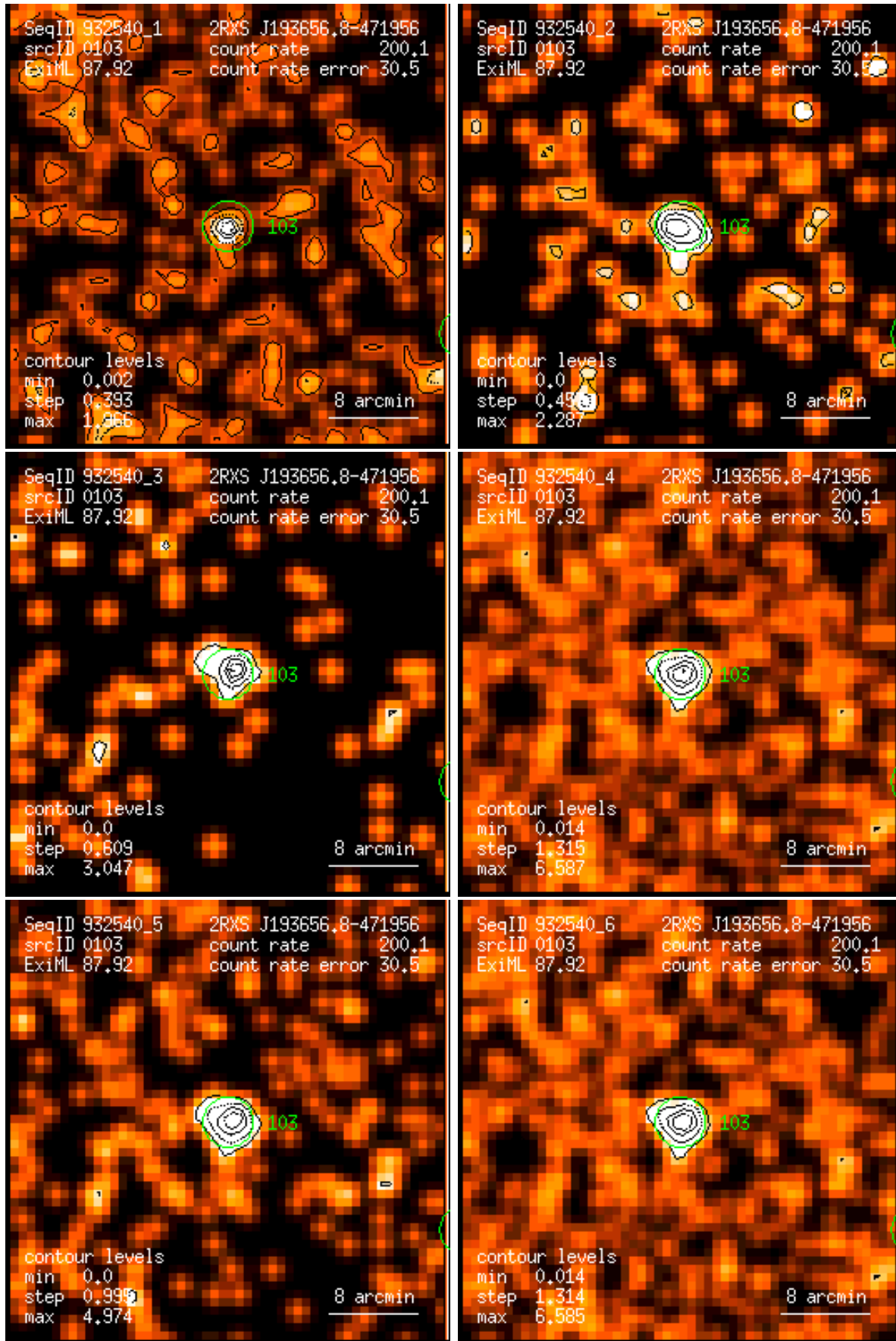
Figure 103: RASS 932540: detection 0103: band rate images, Gaussian filter: (1) PSPC channels 11 – 41, (2) 52 – 90, (3) 91 – 201, (4) 11 – 235, (5) 52 – 201, (6) 11 – 201. Broad band rates in counts/ks. Band rate contour levels in counts/ks/arcmin 2 .
