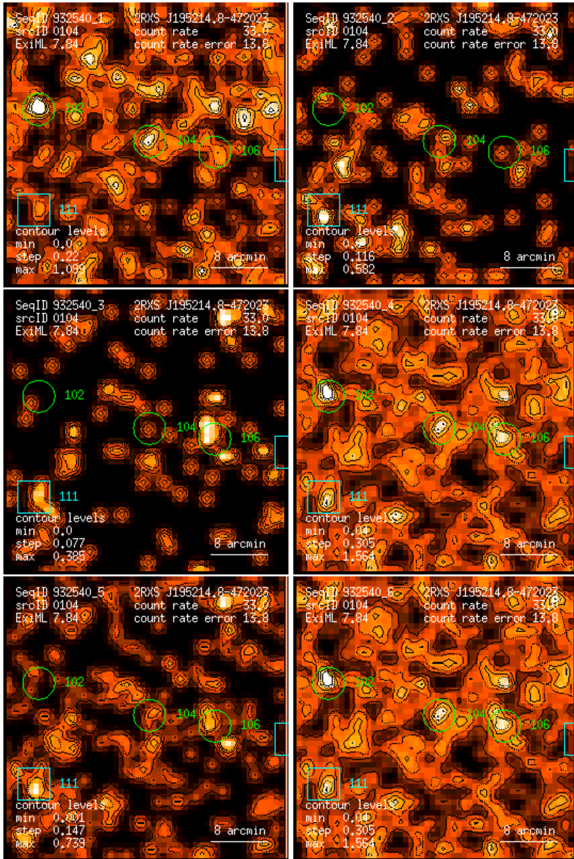
Figure 104: RASS 932540: detection 0104: band rate images, Gaussian filter: (1) PSPC channels 11 – 41, (2) 52 – 90, (3) 91 – 201, (4) 11 – 235, (5) 52 – 201, (6) 11 – 201. Broad band rates in counts/ks. Band rate contour levels in counts/ks/arcmin 2 .
