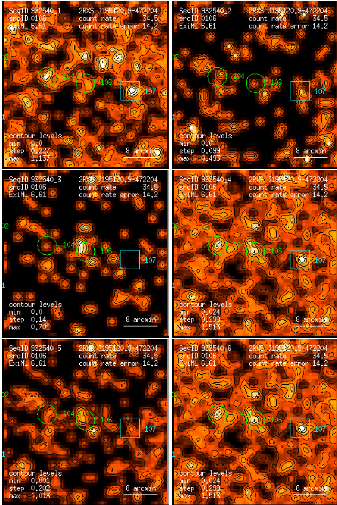
Figure 106: RASS 932540: detection 0106: band rate images, Gaussian filter: (1) PSPC channels 11 – 41, (2) 52 – 90, (3) 91 – 201, (4) 11 – 235, (5) 52 – 201, (6) 11 – 201. Broad band rates in counts/ks. Band rate contour levels in counts/ks/arcmin 2 .
