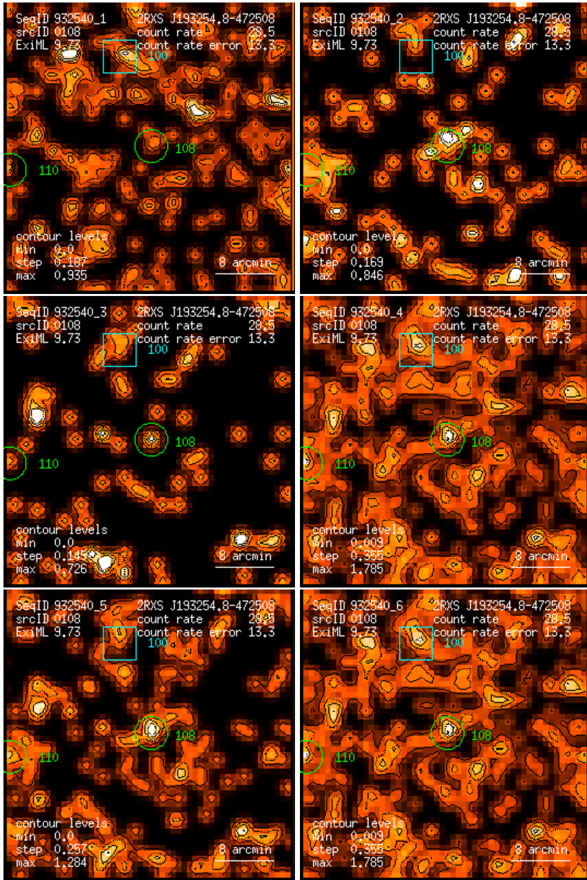
Figure 108: RASS 932540: detection 0108: band rate images, Gaussian filter: (1) PSPC channels 11 – 41, (2) 52 – 90, (3) 91 – 201, (4) 11 – 235, (5) 52 – 201, (6) 11 – 201. Broad band rates in counts/ks. Band rate contour levels in counts/ks/arcmin 2 .
