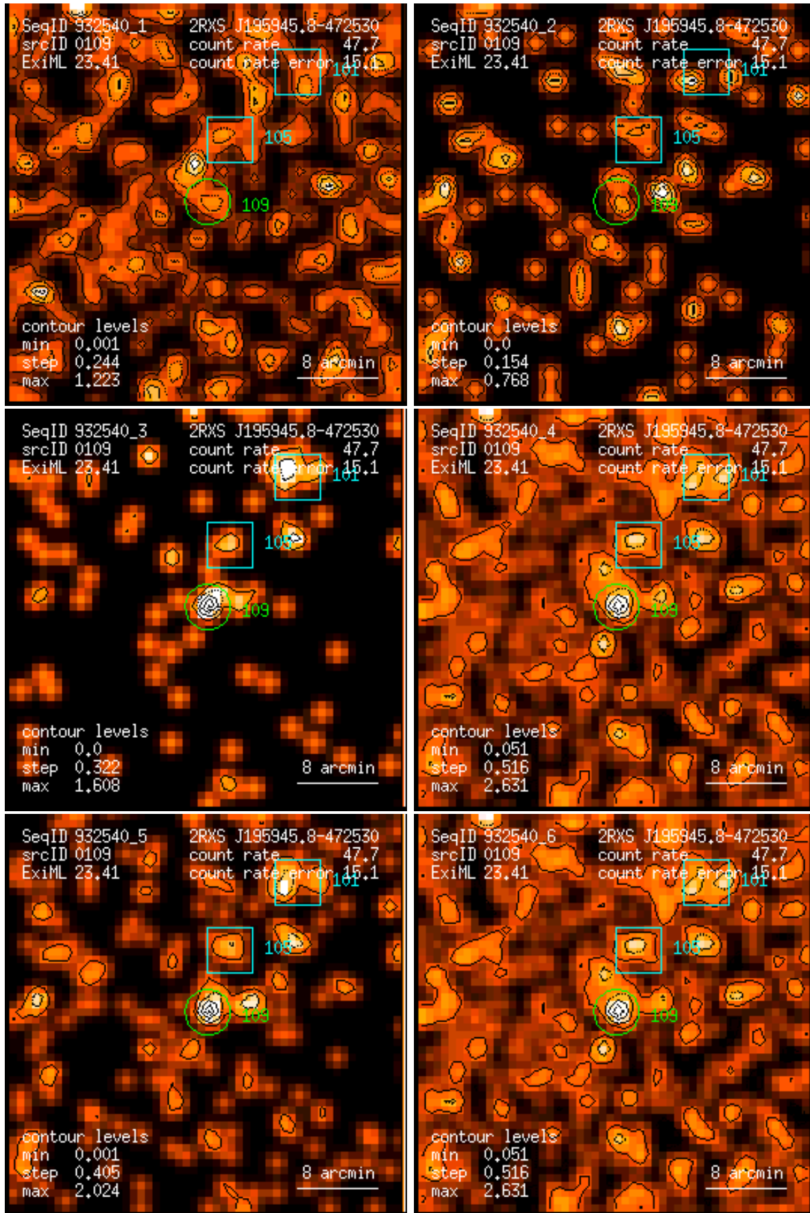
Figure 109: RASS 932540: detection 0109: band rate images, Gaussian filter: (1) PSPC channels 11 – 41, (2) 52 – 90, (3) 91 – 201, (4) 11 – 235, (5) 52 – 201, (6) 11 – 201. Broad band rates in counts/ks. Band rate contour levels in counts/ks/arcmin 2 .
