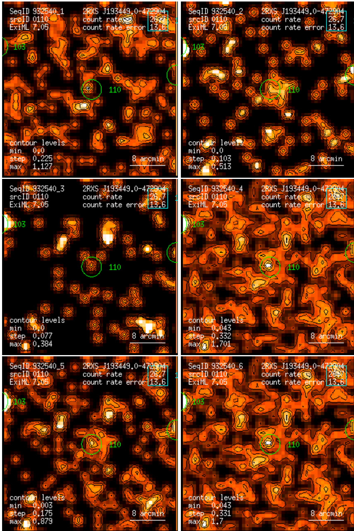
Figure 110: RASS 932540: detection 0110: band rate images, Gaussian filter: (1) PSPC channels 11 – 41, (2) 52 – 90, (3) 91 – 201, (4) 11 – 235, (5) 52 – 201, (6) 11 – 201. Broad band rates in counts/ks. Band rate contour levels in counts/ks/arcmin 2 .
