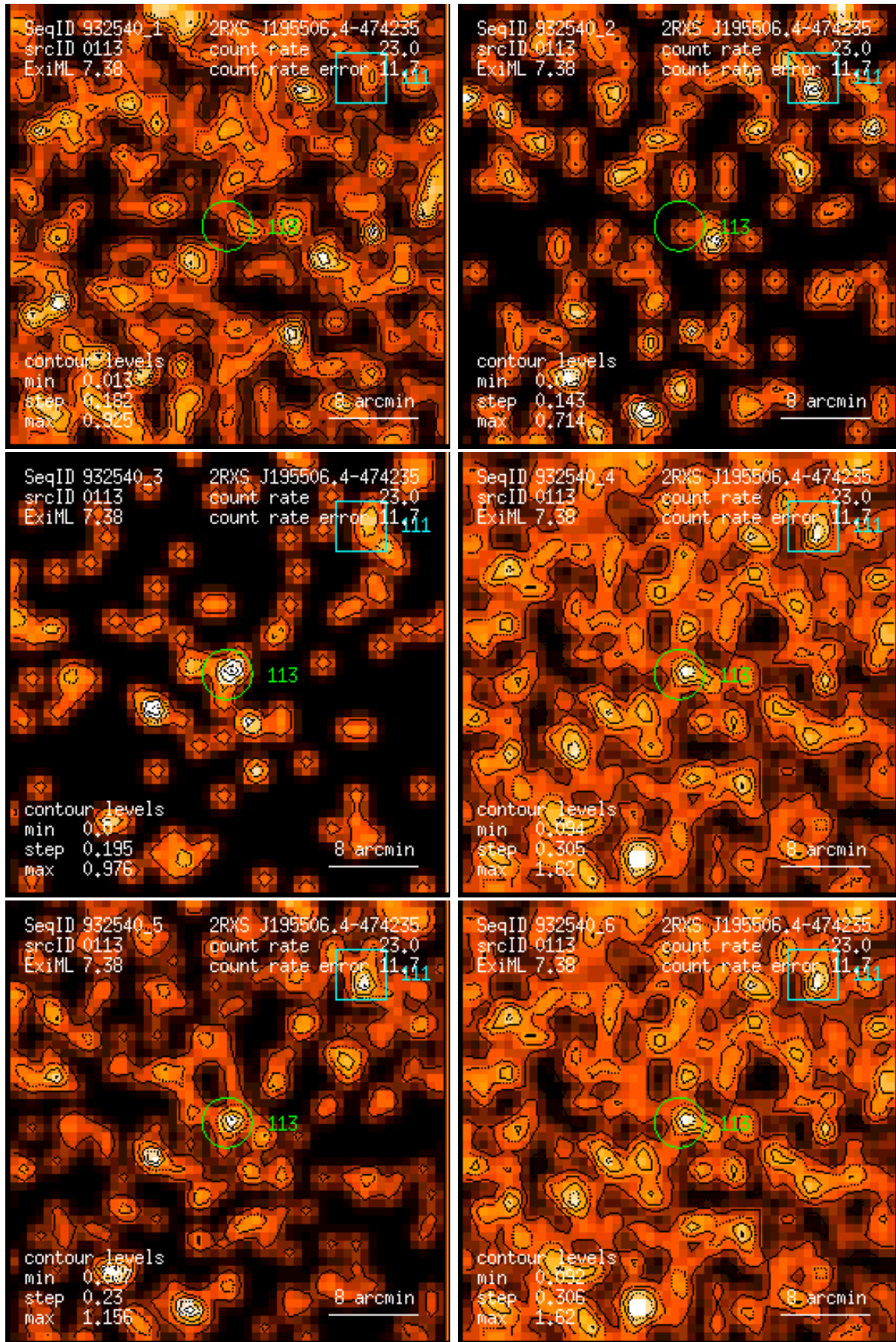
Figure 113: RASS 932540: detection 0113: band rate images, Gaussian filter: (1) PSPC channels 11 – 41, (2) 52 – 90, (3) 91 – 201, (4) 11 – 235, (5) 52 – 201, (6) 11 – 201. Broad band rates in counts/ks. Band rate contour levels in counts/ks/arcmin 2 .
