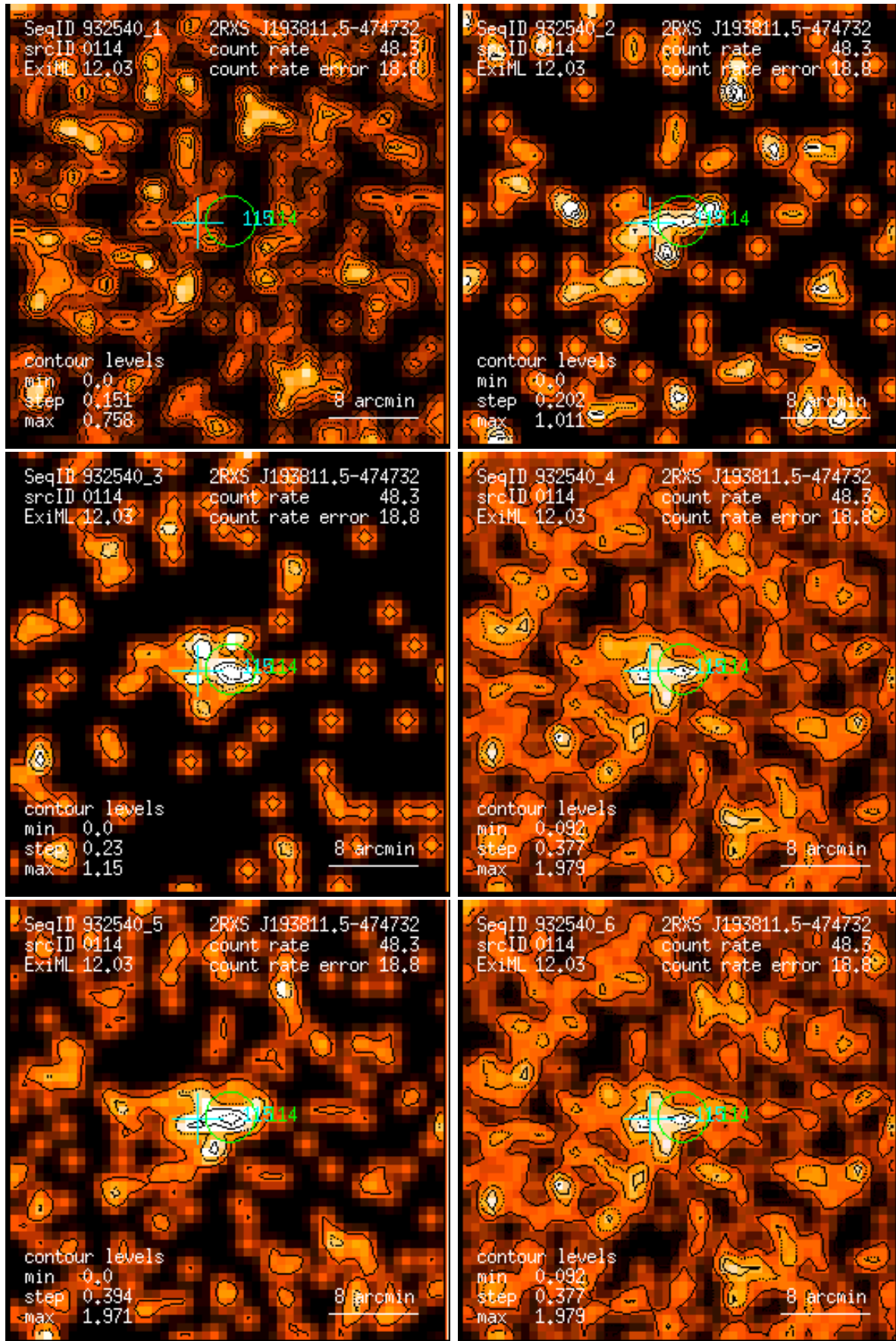
Figure 114: RASS 932540: detection 0114: band rate images, Gaussian filter: (1) PSPC channels 11 – 41, (2) 52 – 90, (3) 91 – 201, (4) 11 – 235, (5) 52 – 201, (6) 11 – 201. Broad band rates in counts/ks. Band rate contour levels in counts/ks/arcmin 2 .
