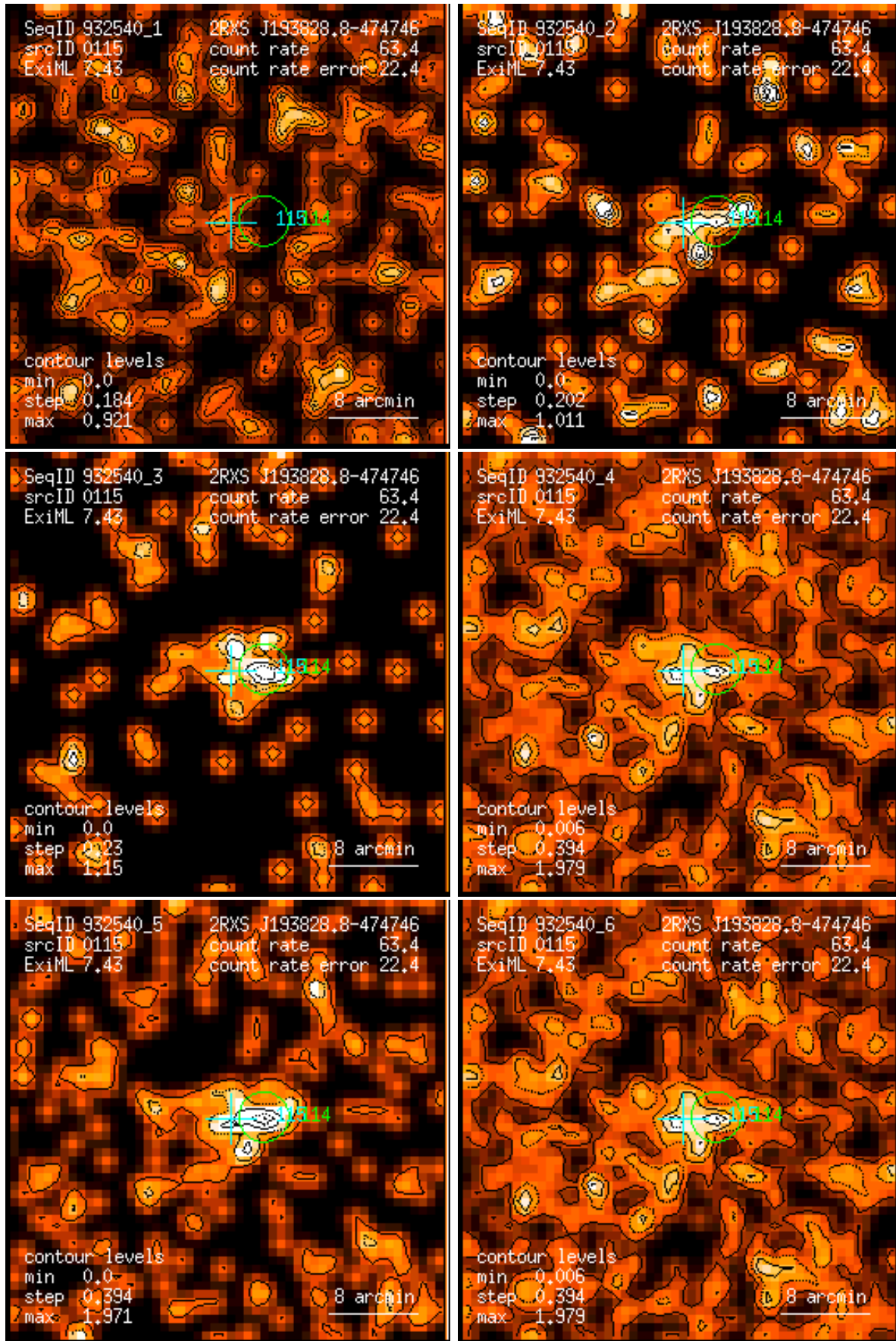
Figure 115: RASS 932540: detection 0115: band rate images, Gaussian filter: (1) PSPC channels 11 – 41, (2) 52 – 90, (3) 91 – 201, (4) 11 – 235, (5) 52 – 201, (6) 11 – 201. Broad band rates in counts/ks. Band rate contour levels in counts/ks/arcmin 2 .
