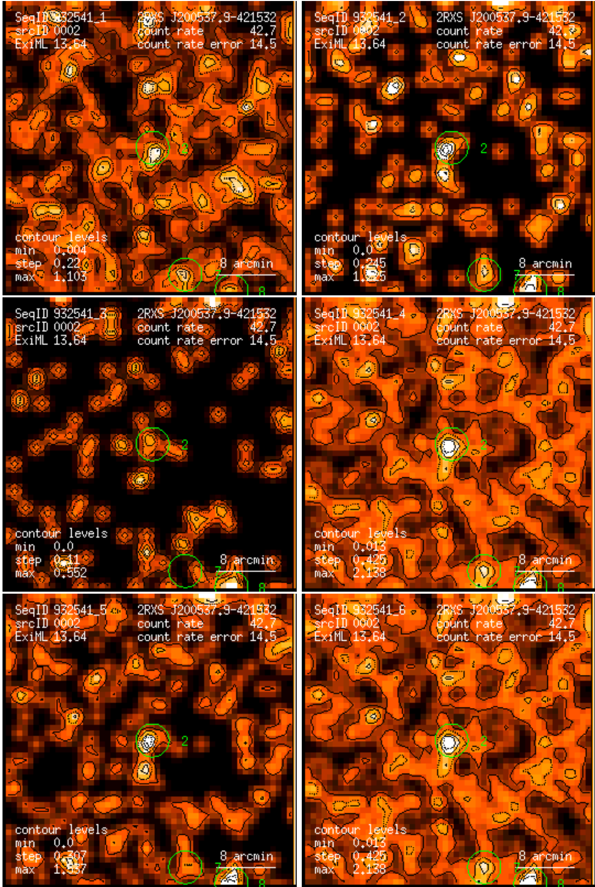
Figure 2: RASS 932541: detection 0002: band rate images, Gaussian filter: (1) PSPC channels 11 – 41, (2) 52 – 90, (3) 91 – 201, (4) 11 – 235, (5) 52 – 201, (6) 11 – 201. Broad band rates in counts/ks. Band rate contour levels in counts/ks/arcmin 2 .
