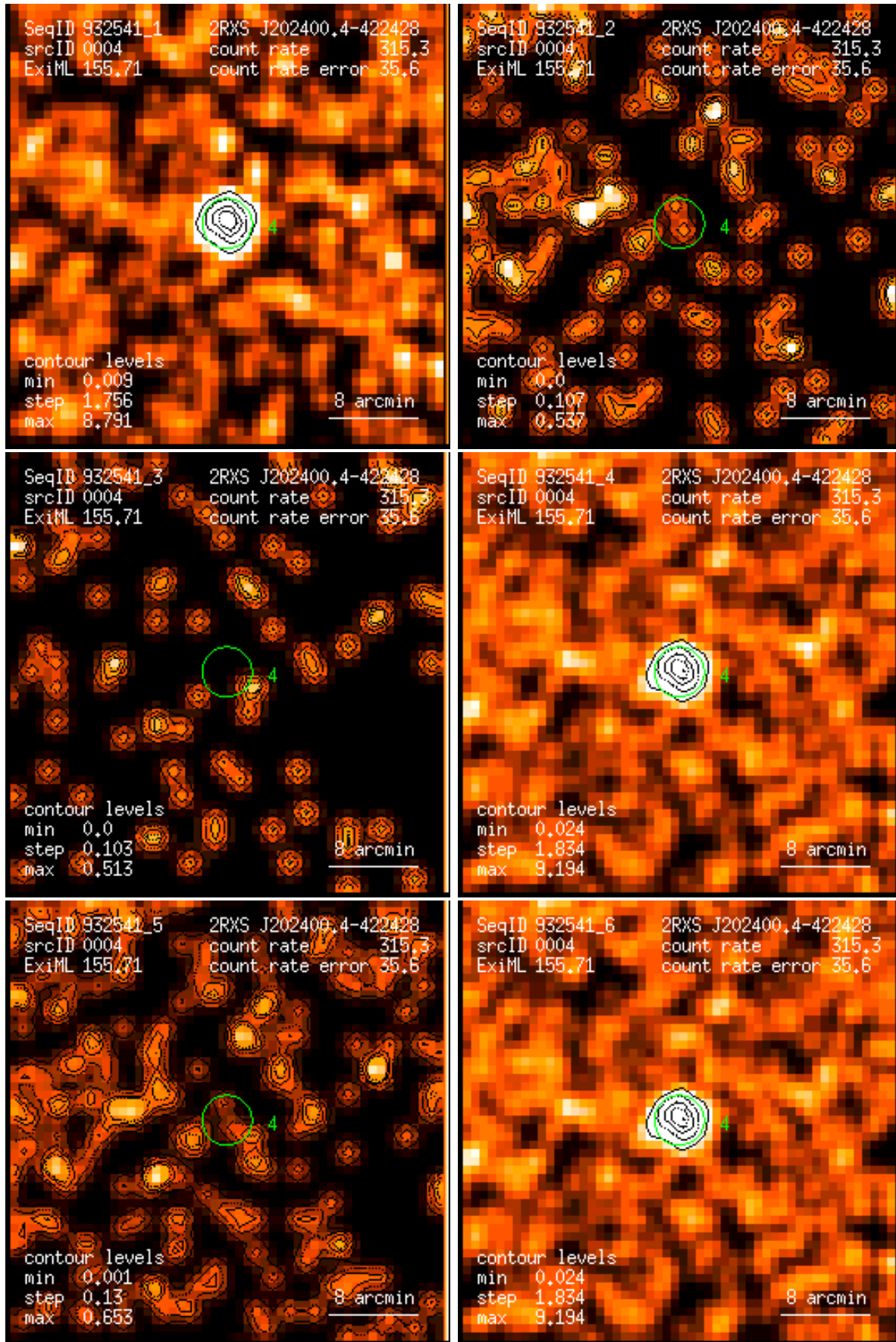
Figure 4: RASS 932541: detection 0004: band rate images, Gaussian filter: (1) PSPC channels 11 – 41, (2) 52 – 90, (3) 91 – 201, (4) 11 – 235, (5) 52 – 201, (6) 11 – 201. Broad band rates in counts/ks. Band rate contour levels in counts/ks/arcmin 2 .
