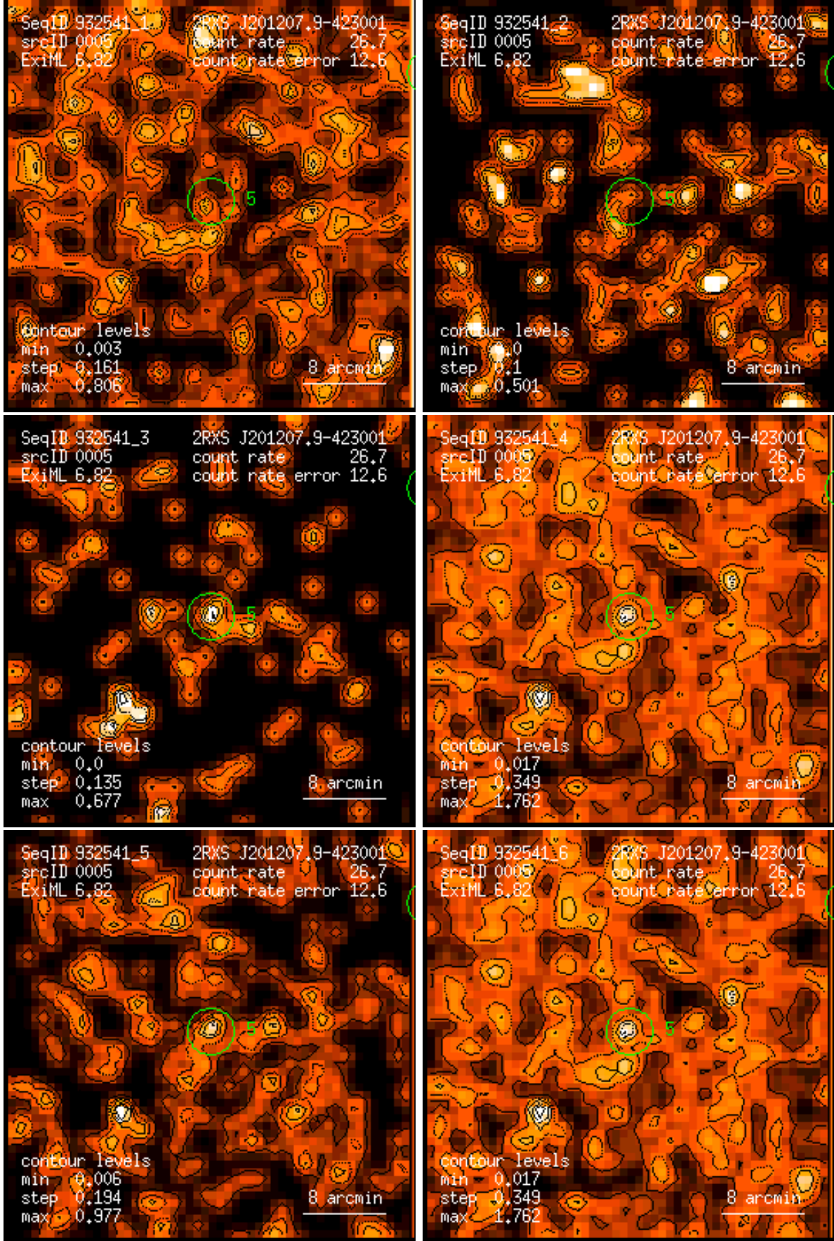
Figure 5: RASS 932541: detection 0005: band rate images, Gaussian filter: (1) PSPC channels 11 – 41, (2) 52 – 90, (3) 91 – 201, (4) 11 – 235, (5) 52 – 201, (6) 11 – 201. Broad band rates in counts/ks. Band rate contour levels in counts/ks/arcmin 2 .
