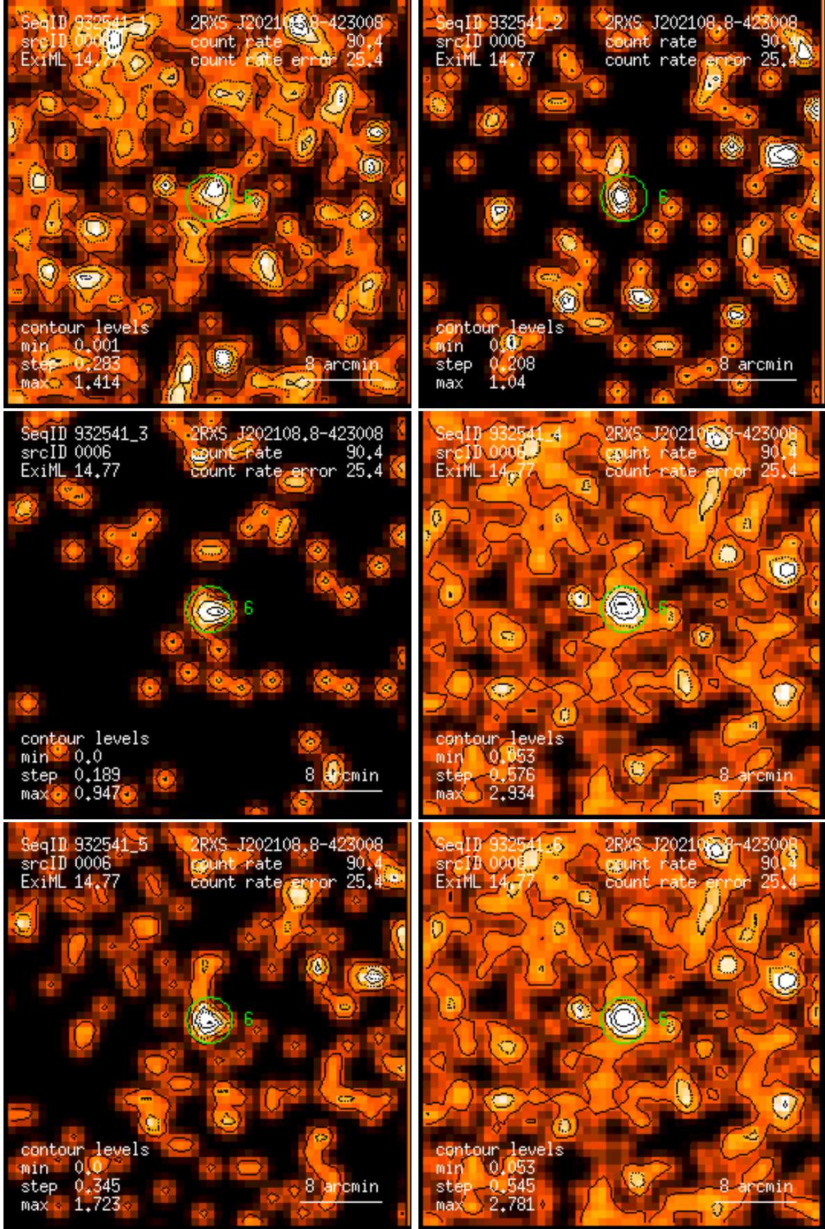
Figure 6: RASS 932541: detection 0006: band rate images, Gaussian filter: (1) PSPC channels 11 – 41, (2) 52 – 90, (3) 91 – 201, (4) 11 – 235, (5) 52 – 201, (6) 11 – 201. Broad band rates in counts/ks. Band rate contour levels in counts/ks/arcmin 2 .
