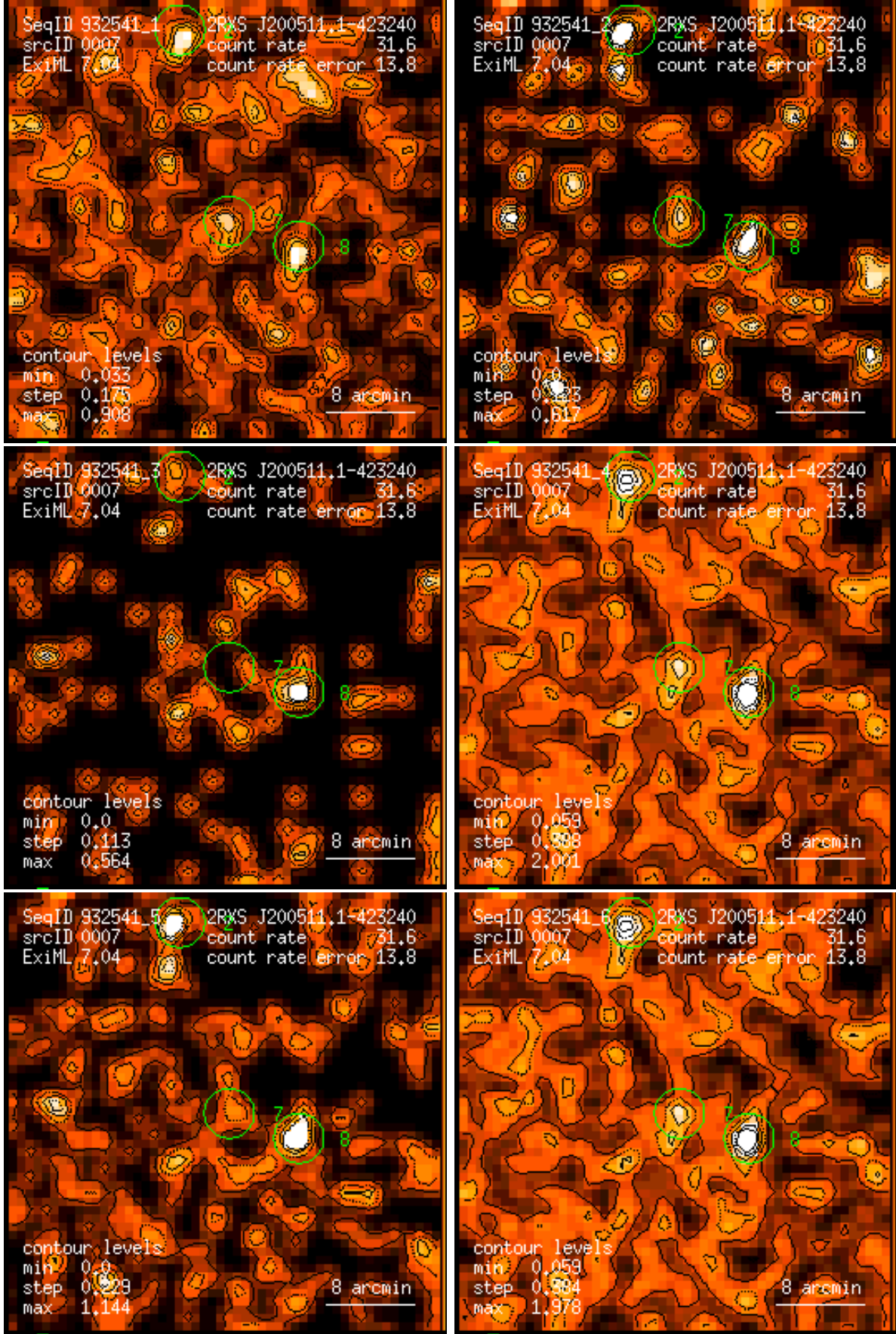
Figure 7: RASS 932541: detection 0007: band rate images, Gaussian filter: (1) PSPC channels 11 – 41, (2) 52 – 90, (3) 91 – 201, (4) 11 – 235, (5) 52 – 201, (6) 11 – 201. Broad band rates in counts/ks. Band rate contour levels in counts/ks/arcmin 2 .
