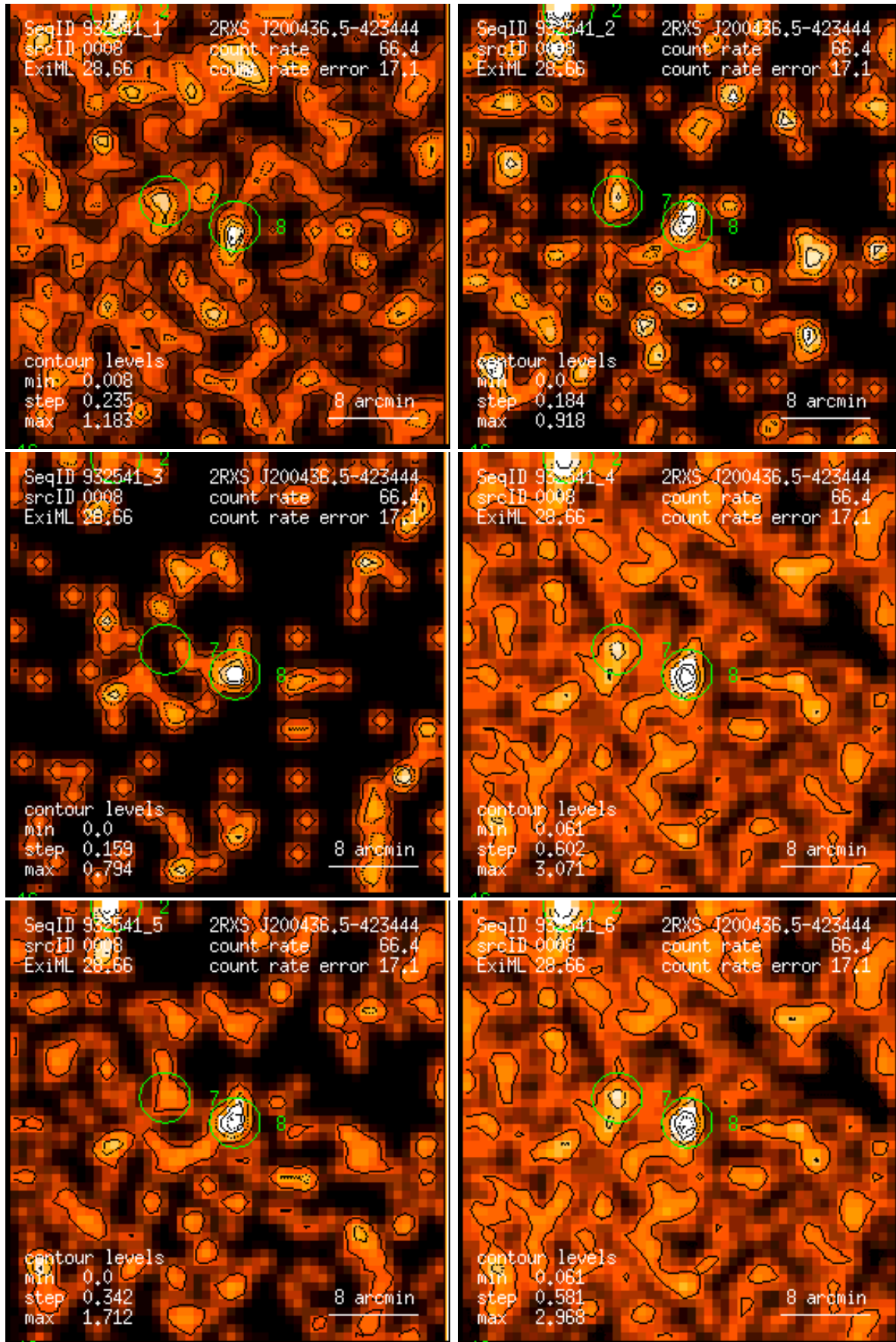
Figure 8: RASS 932541: detection 0008: band rate images, Gaussian filter: (1) PSPC channels 11 – 41, (2) 52 – 90, (3) 91 – 201, (4) 11 – 235, (5) 52 – 201, (6) 11 – 201. Broad band rates in counts/ks. Band rate contour levels in counts/ks/arcmin 2 .
