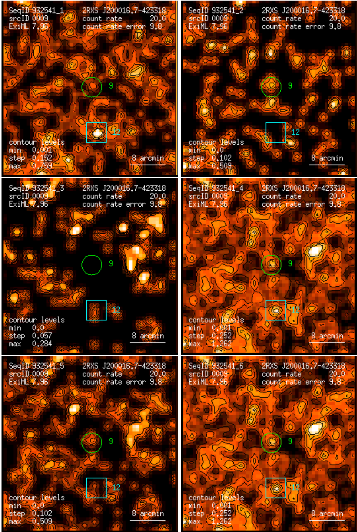
Figure 9: RASS 932541: detection 0009: band rate images, Gaussian filter: (1) PSPC channels 11 – 41, (2) 52 – 90, (3) 91 – 201, (4) 11 – 235, (5) 52 – 201, (6) 11 – 201. Broad band rates in counts/ks. Band rate contour levels in counts/ks/arcmin 2 .
