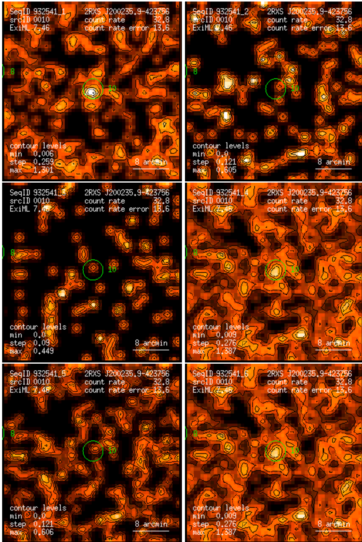
Figure 10: RASS 932541: detection 0010: band rate images, Gaussian filter: (1) PSPC channels 11 – 41, (2) 52 – 90, (3) 91 – 201, (4) 11 – 235, (5) 52 – 201, (6) 11 – 201. Broad band rates in counts/ks. Band rate contour levels in counts/ks/arcmin 2 .
