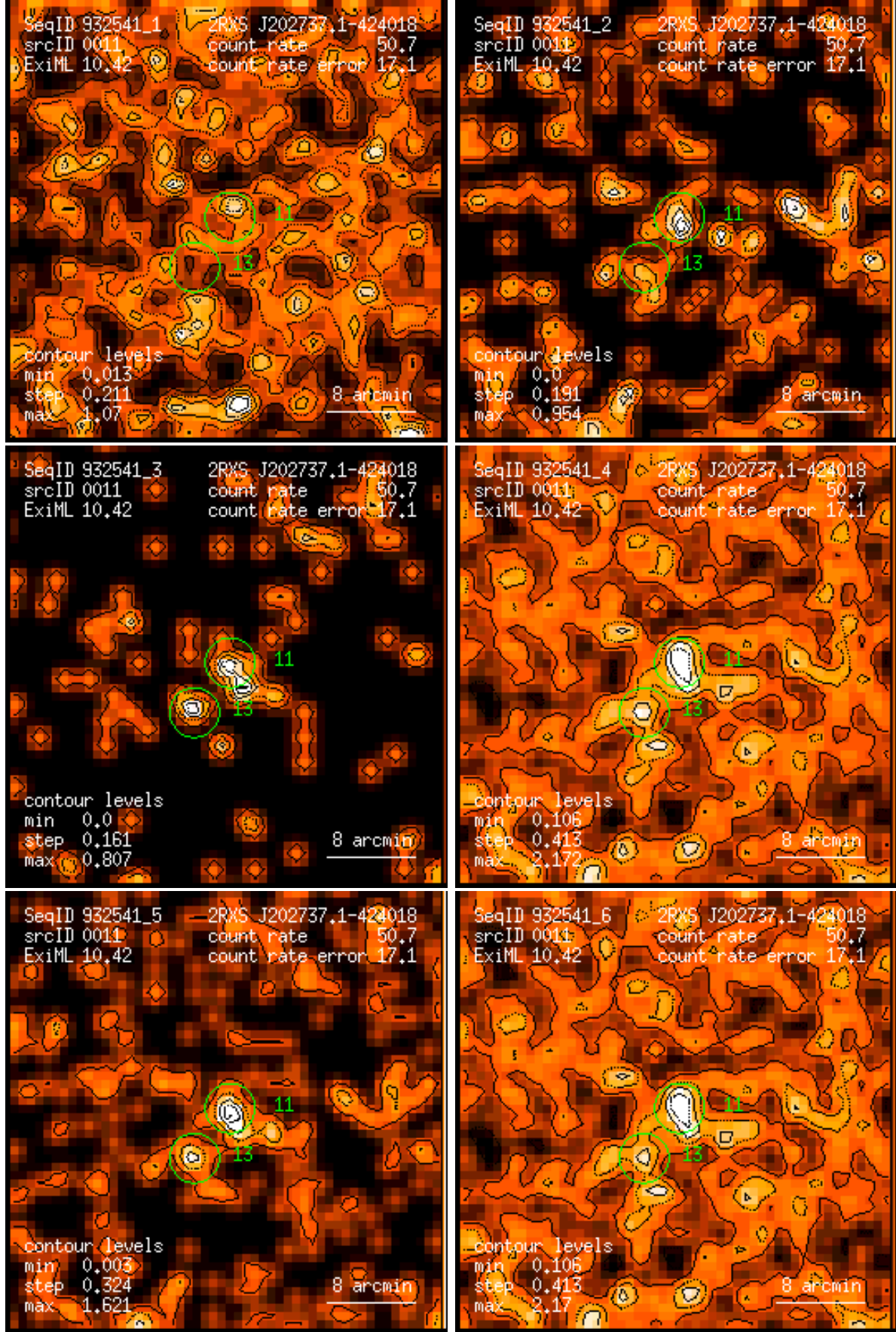
Figure 11: RASS 932541: detection 0011: band rate images, Gaussian filter: (1) PSPC channels 11 – 41, (2) 52 – 90, (3) 91 – 201, (4) 11 – 235, (5) 52 – 201, (6) 11 – 201. Broad band rates in counts/ks. Band rate contour levels in counts/ks/arcmin 2 .
