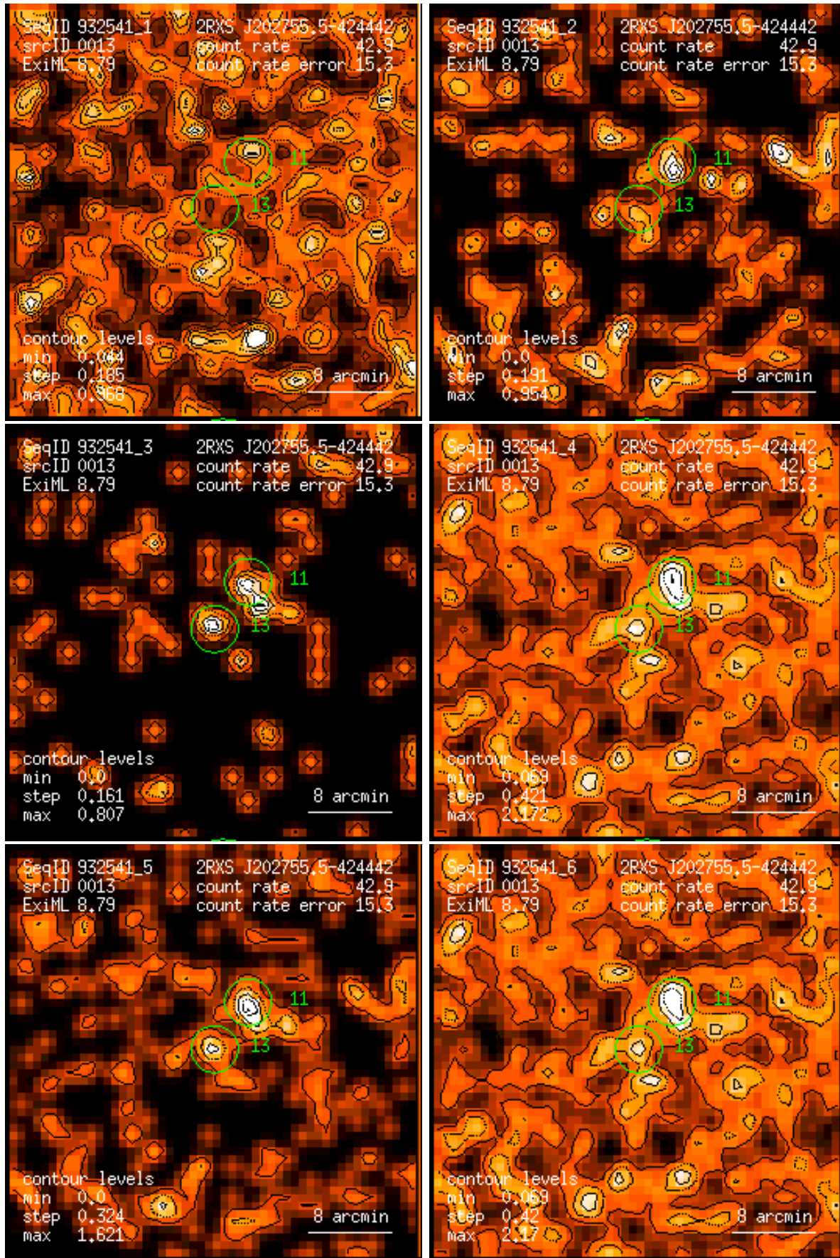
Figure 13: RASS 932541: detection 0013: band rate images, Gaussian filter: (1) PSPC channels 11 – 41, (2) 52 – 90, (3) 91 – 201, (4) 11 – 235, (5) 52 – 201, (6) 11 – 201. Broad band rates in counts/ks. Band rate contour levels in counts/ks/arcmin 2 .
