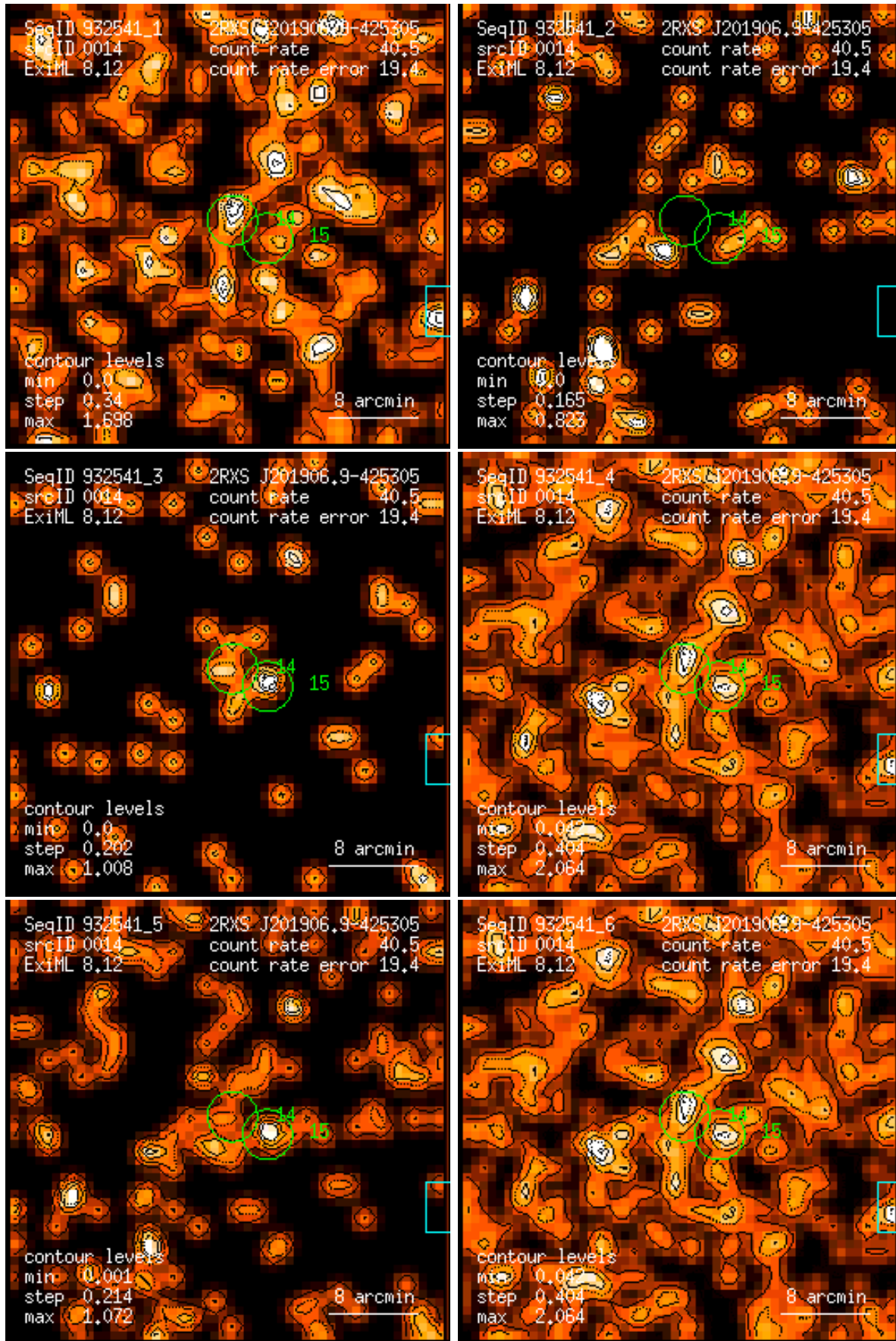
Figure 14: RASS 932541: detection 0014: band rate images, Gaussian filter: (1) PSPC channels 11 – 41, (2) 52 – 90, (3) 91 – 201, (4) 11 – 235, (5) 52 – 201, (6) 11 – 201. Broad band rates in counts/ks. Band rate contour levels in counts/ks/arcmin 2 .
