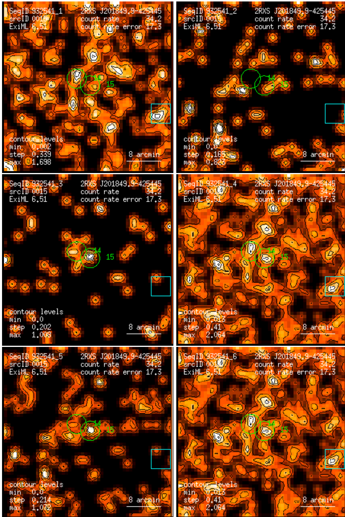
Figure 15: RASS 932541: detection 0015: band rate images, Gaussian filter: (1) PSPC channels 11 – 41, (2) 52 – 90, (3) 91 – 201, (4) 11 – 235, (5) 52 – 201, (6) 11 – 201. Broad band rates in counts/ks. Band rate contour levels in counts/ks/arcmin 2 .
