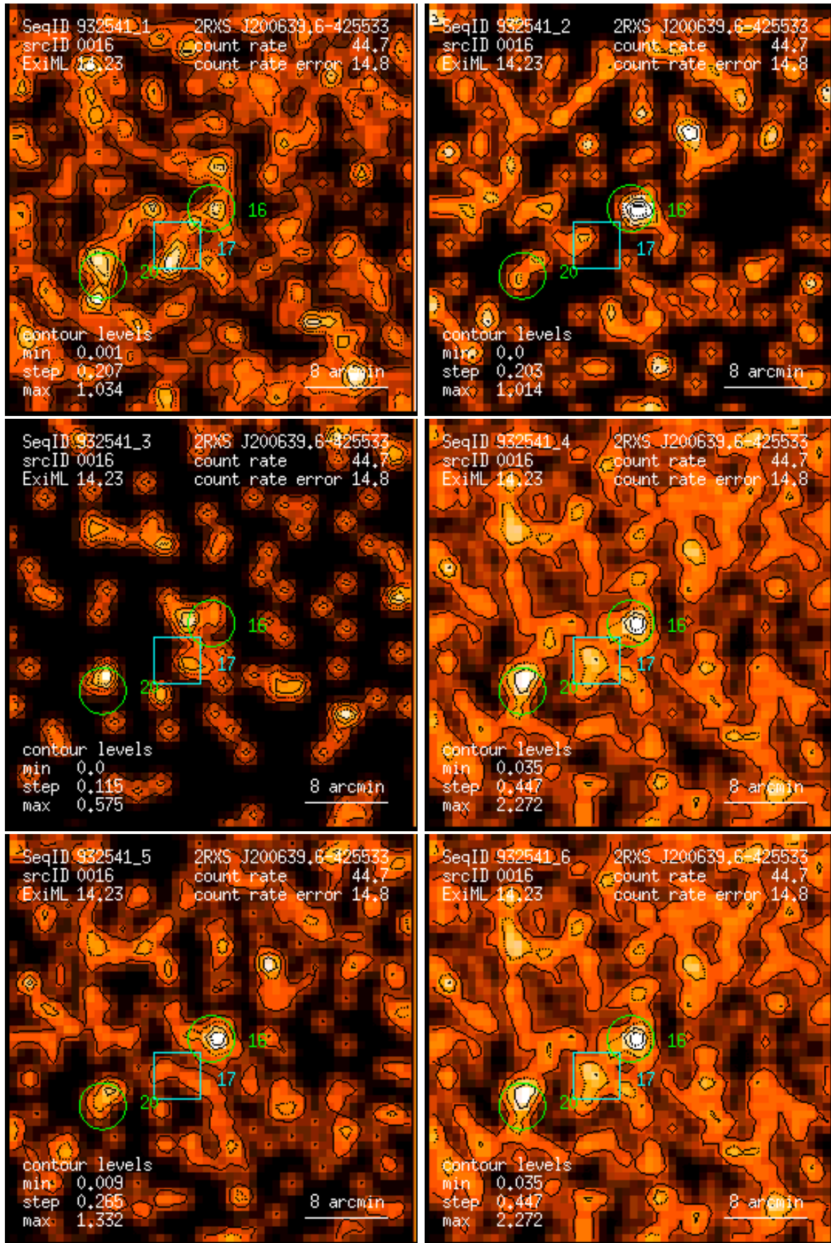
Figure 16: RASS 932541: detection 0016: band rate images, Gaussian filter: (1) PSPC channels 11 – 41, (2) 52 – 90, (3) 91 – 201, (4) 11 – 235, (5) 52 – 201, (6) 11 – 201. Broad band rates in counts/ks. Band rate contour levels in counts/ks/arcmin 2 .
