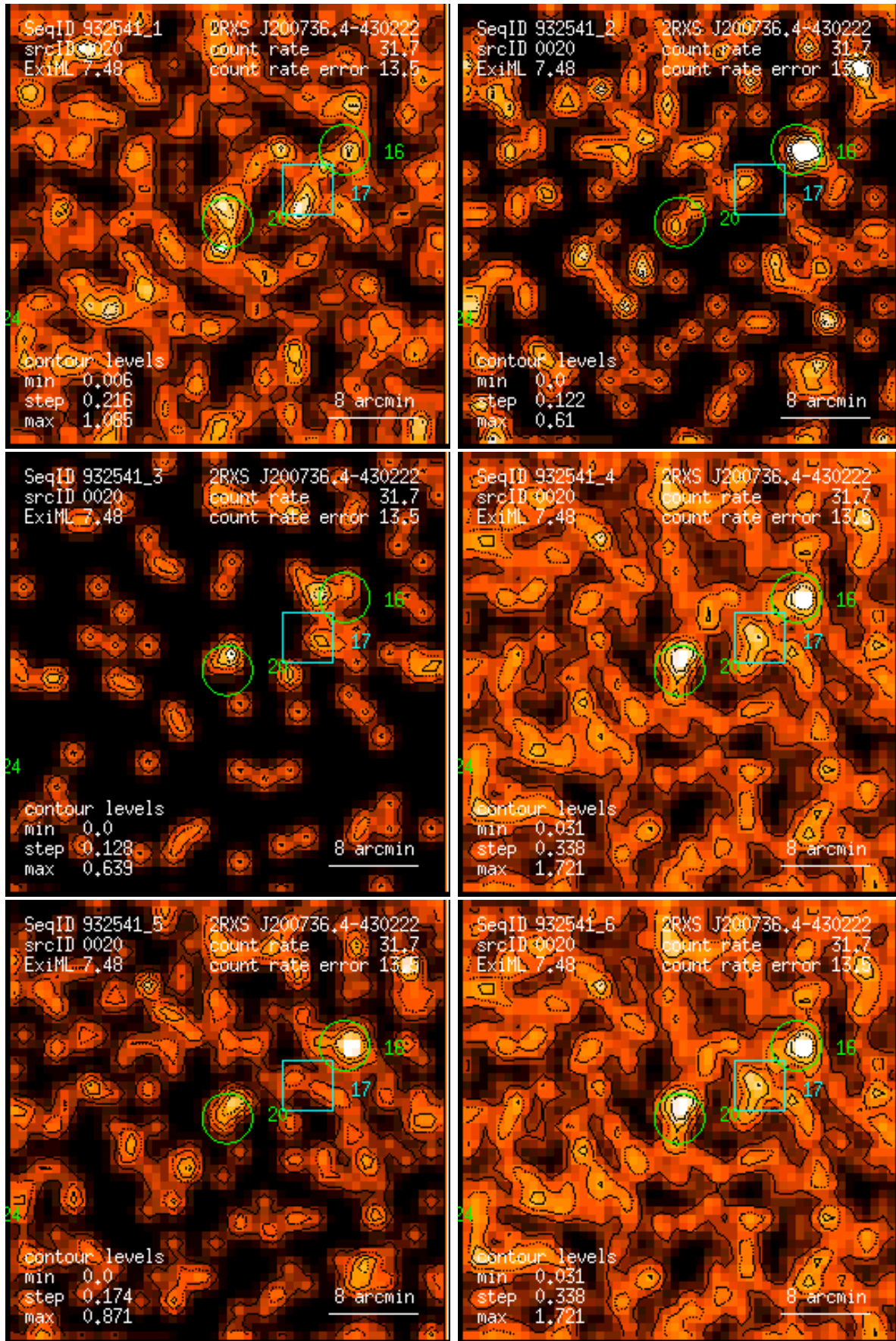
Figure 20: RASS 932541: detection 0020: band rate images, Gaussian filter: (1) PSPC channels 11 – 41, (2) 52 – 90, (3) 91 – 201, (4) 11 – 235, (5) 52 – 201, (6) 11 – 201. Broad band rates in counts/ks. Band rate contour levels in counts/ks/arcmin 2 .
