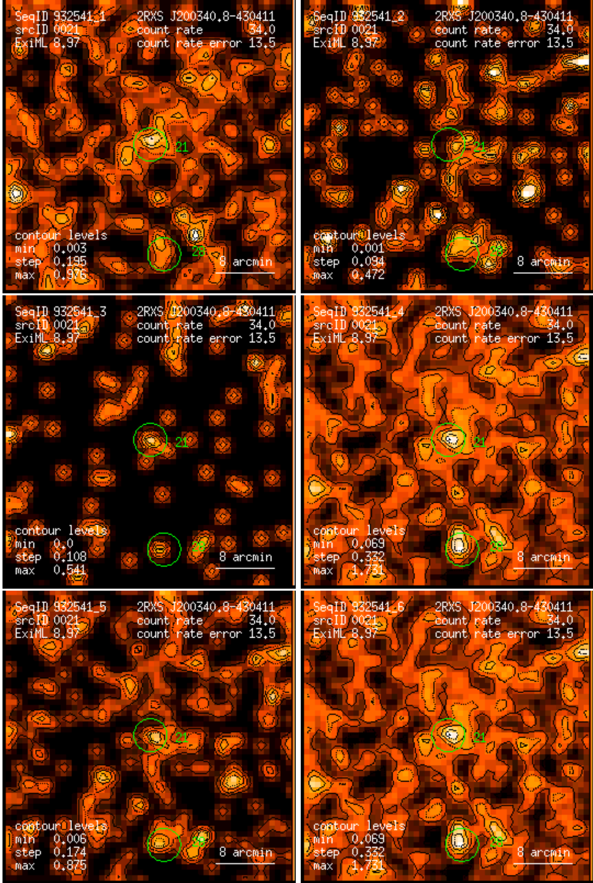
Figure 21: RASS 932541: detection 0021: band rate images, Gaussian filter: (1) PSPC channels 11 – 41, (2) 52 – 90, (3) 91 – 201, (4) 11 – 235, (5) 52 – 201, (6) 11 – 201. Broad band rates in counts/ks. Band rate contour levels in counts/ks/arcmin 2 .
