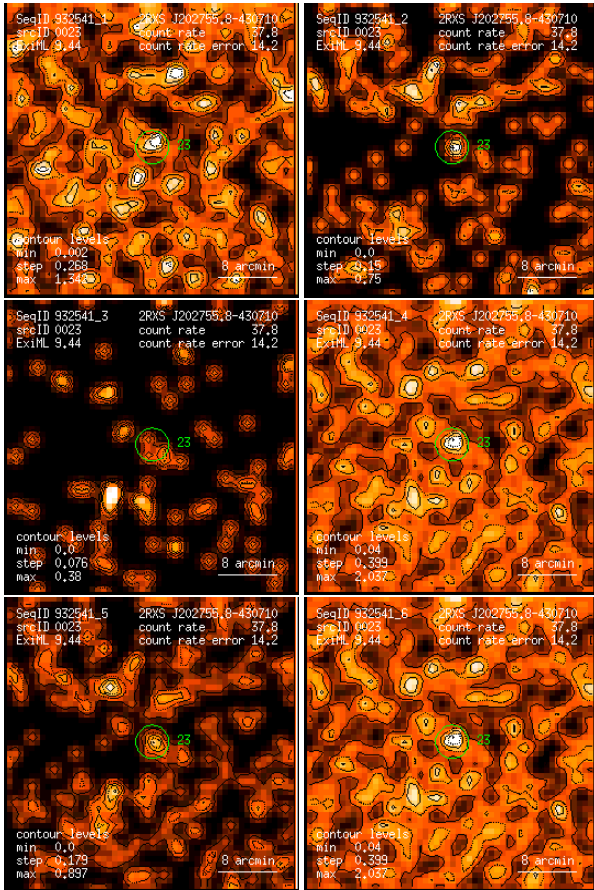
Figure 23: RASS 932541: detection 0023: band rate images, Gaussian filter: (1) PSPC channels 11 – 41, (2) 52 – 90, (3) 91 – 201, (4) 11 – 235, (5) 52 – 201, (6) 11 – 201. Broad band rates in counts/ks. Band rate contour levels in counts/ks/arcmin 2 .
