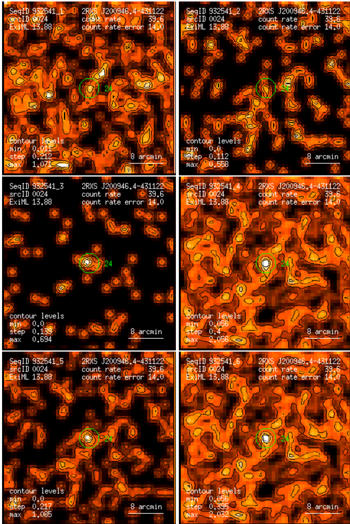
Figure 24: RASS 932541: detection 0024: band rate images, Gaussian filter: (1) PSPC channels 11 – 41, (2) 52 – 90, (3) 91 – 201, (4) 11 – 235, (5) 52 – 201, (6) 11 – 201. Broad band rates in counts/ks. Band rate contour levels in counts/ks/arcmin 2 .
