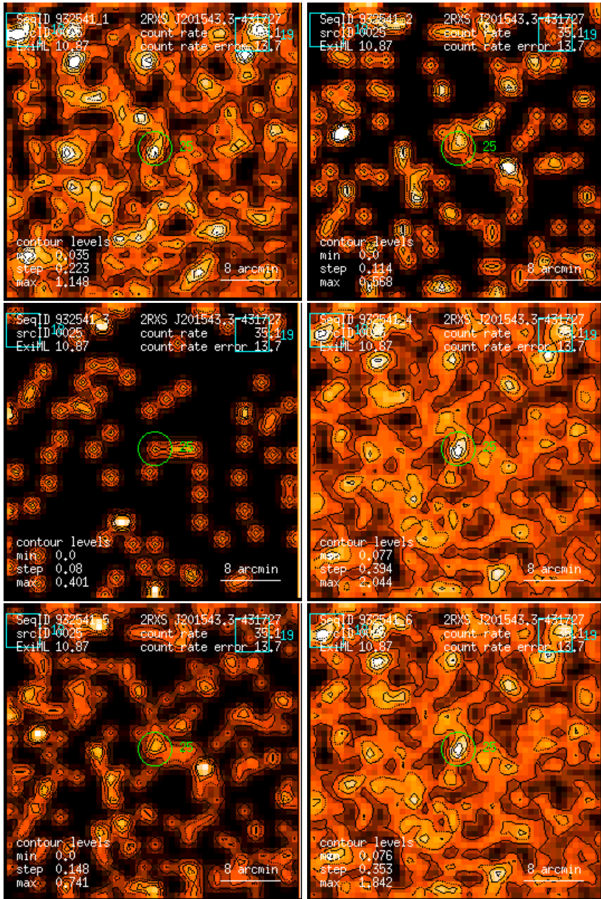
Figure 25: RASS 932541: detection 0025: band rate images, Gaussian filter: (1) PSPC channels 11 – 41, (2) 52 – 90, (3) 91 – 201, (4) 11 – 235, (5) 52 – 201, (6) 11 – 201. Broad band rates in counts/ks. Band rate contour levels in counts/ks/arcmin 2 .
