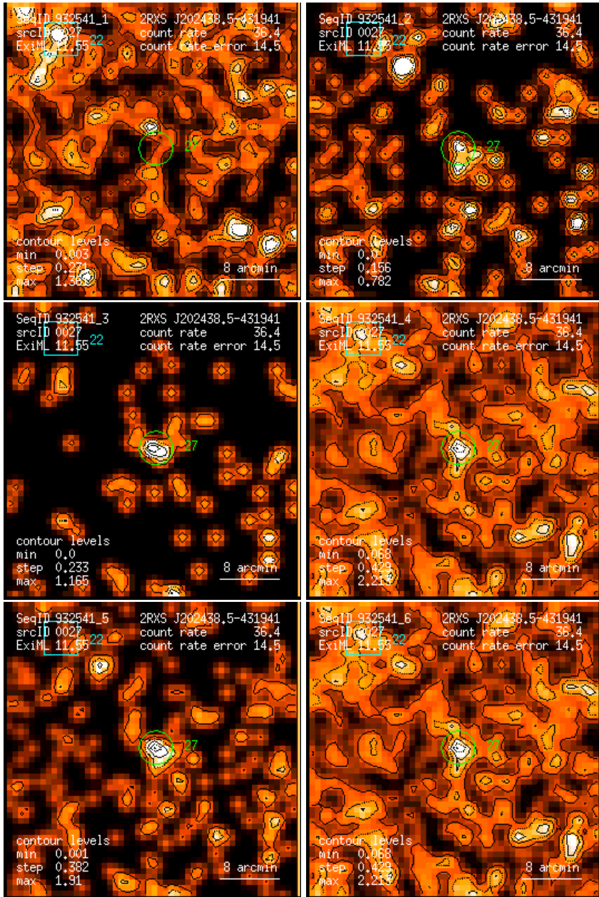
Figure 27: RASS 932541: detection 0027: band rate images, Gaussian filter: (1) PSPC channels 11 – 41, (2) 52 – 90, (3) 91 – 201, (4) 11 – 235, (5) 52 – 201, (6) 11 – 201. Broad band rates in counts/ks. Band rate contour levels in counts/ks/arcmin 2 .
