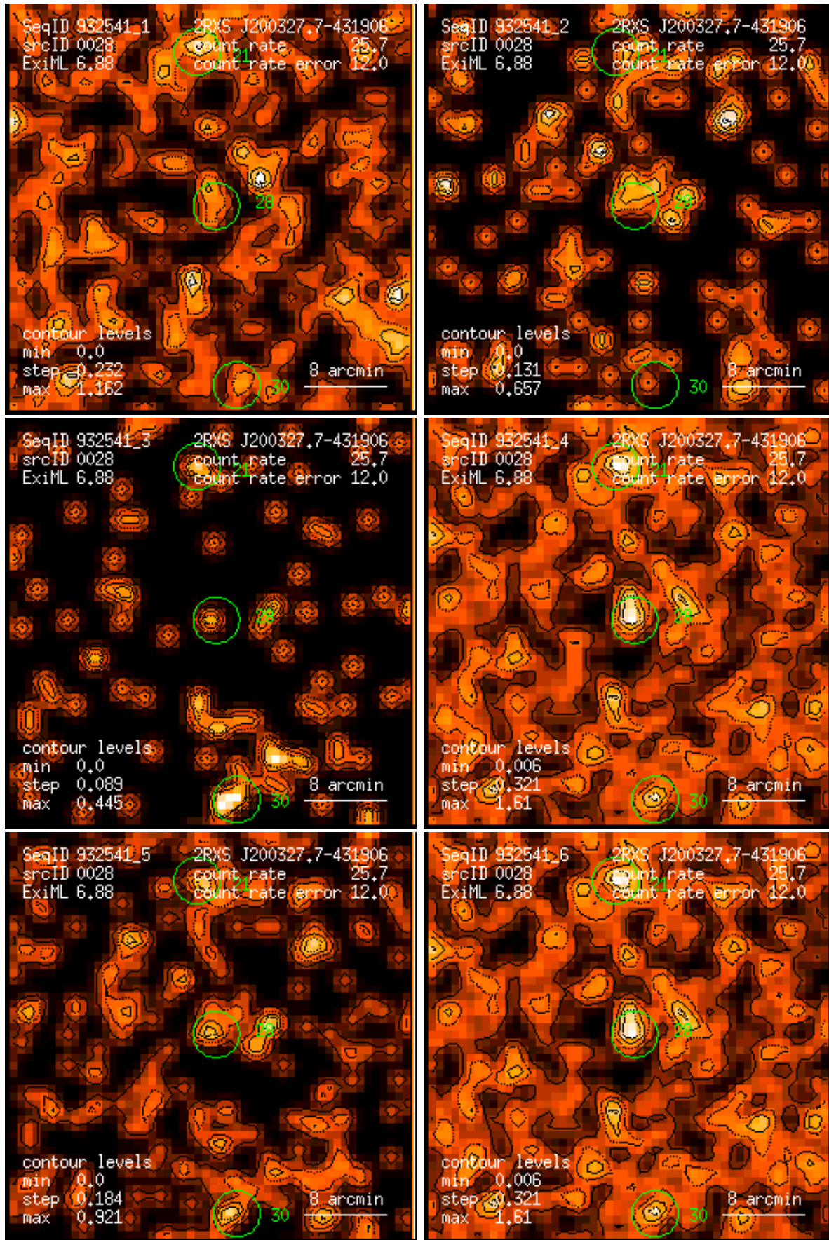
Figure 28: RASS 932541: detection 0028: band rate images, Gaussian filter: (1) PSPC channels 11 – 41, (2) 52 – 90, (3) 91 – 201, (4) 11 – 235, (5) 52 – 201, (6) 11 – 201. Broad band rates in counts/ks. Band rate contour levels in counts/ks/arcmin 2 .
