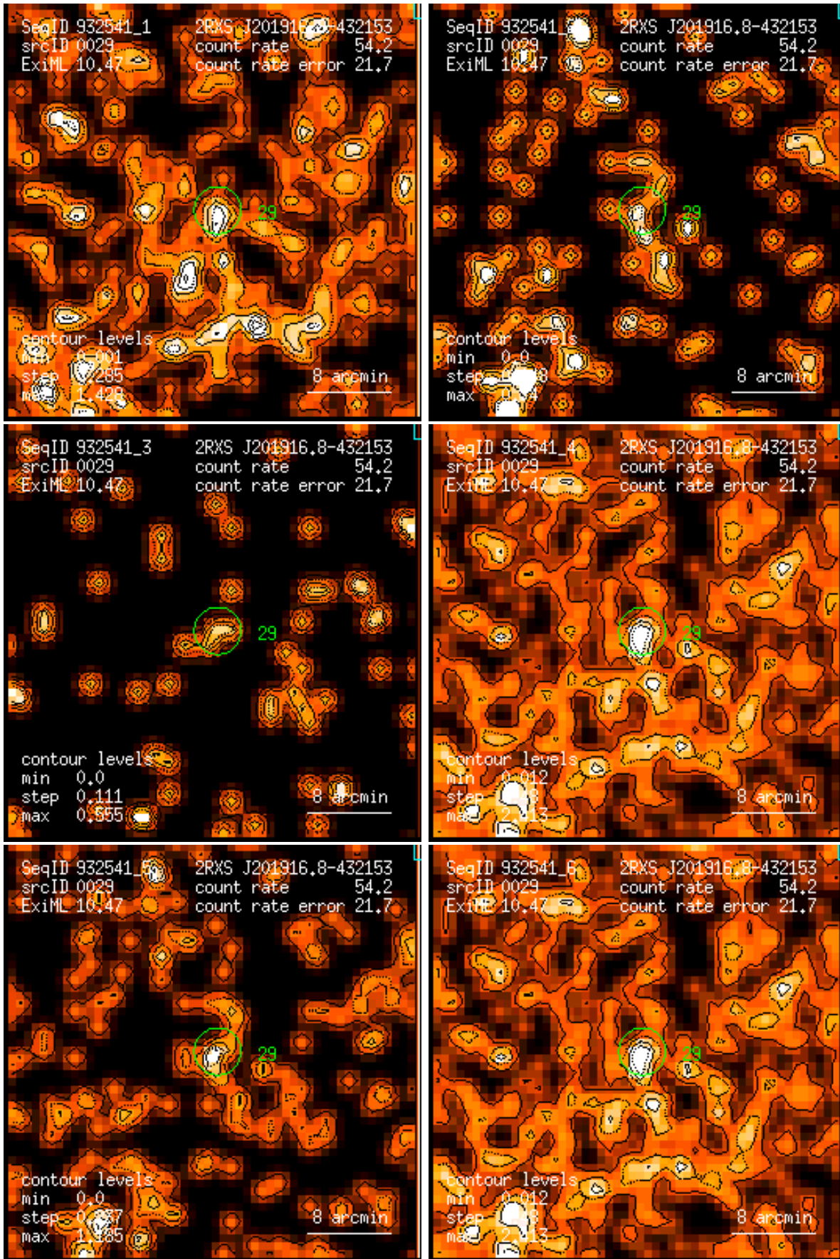
Figure 29: RASS 932541: detection 0029: band rate images, Gaussian filter: (1) PSPC channels 11 – 41, (2) 52 – 90, (3) 91 – 201, (4) 11 – 235, (5) 52 – 201, (6) 11 – 201. Broad band rates in counts/ks. Band rate contour levels in counts/ks/arcmin 2 .
