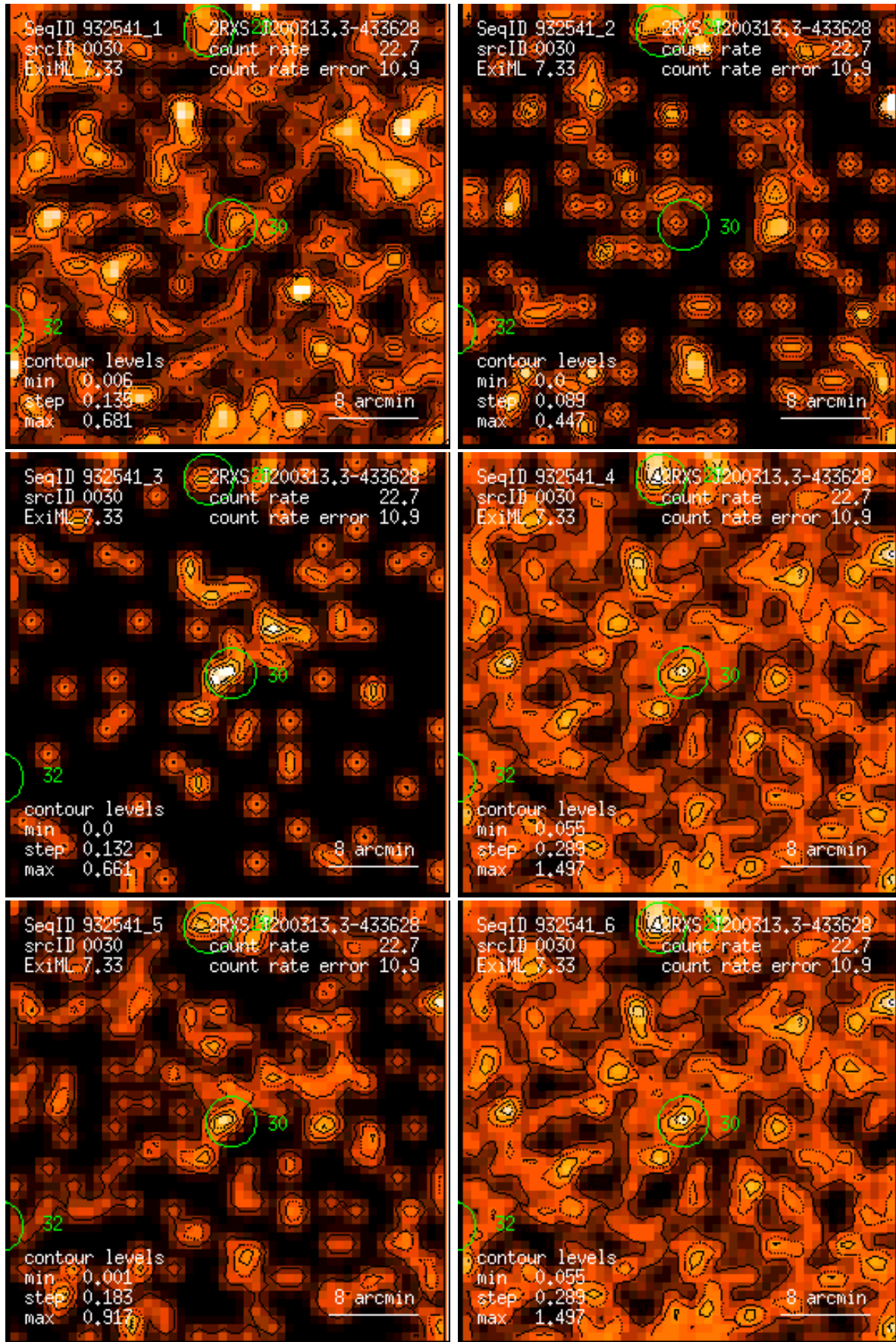
Figure 30: RASS 932541: detection 0030: band rate images, Gaussian filter: (1) PSPC channels 11 – 41, (2) 52 – 90, (3) 91 – 201, (4) 11 – 235, (5) 52 – 201, (6) 11 – 201. Broad band rates in counts/ks. Band rate contour levels in counts/ks/arcmin 2 .
