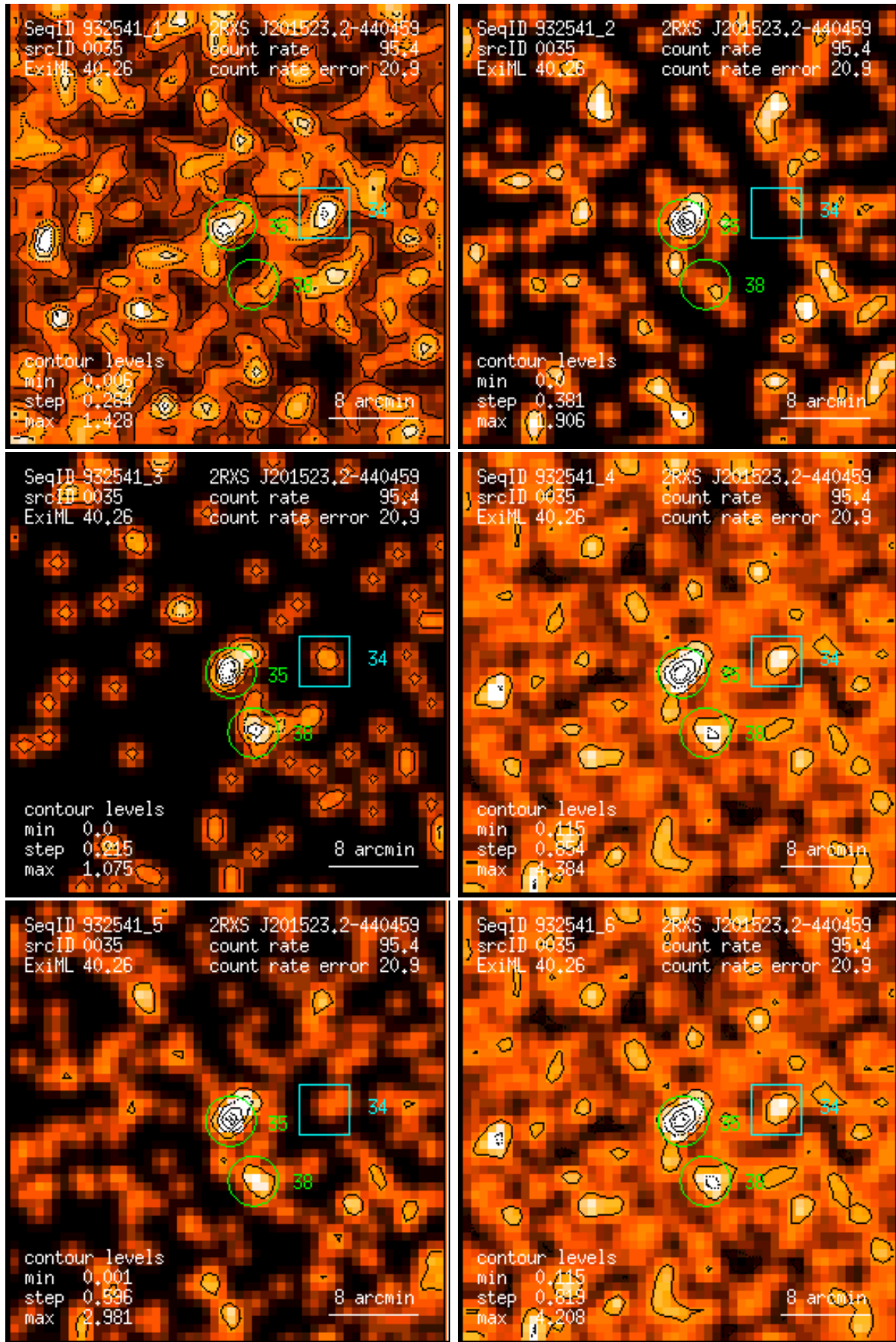
Figure 35: RASS 932541: detection 0035: band rate images, Gaussian filter: (1) PSPC channels 11 – 41, (2) 52 – 90, (3) 91 – 201, (4) 11 – 235, (5) 52 – 201, (6) 11 – 201. Broad band rates in counts/ks. Band rate contour levels in counts/ks/arcmin 2 .
