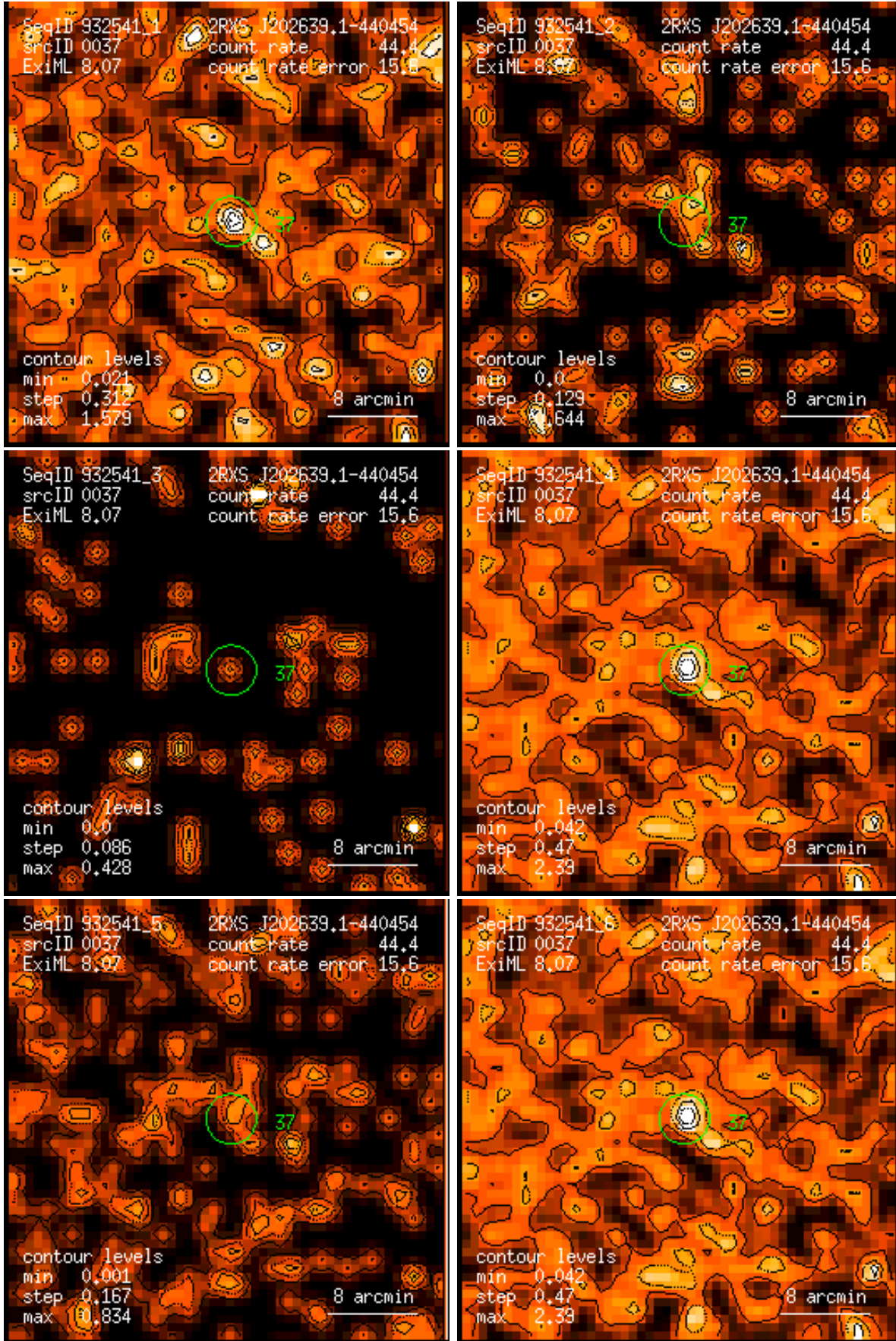
Figure 37: RASS 932541: detection 0037: band rate images, Gaussian filter: (1) PSPC channels 11 – 41, (2) 52 – 90, (3) 91 – 201, (4) 11 – 235, (5) 52 – 201, (6) 11 – 201. Broad band rates in counts/ks. Band rate contour levels in counts/ks/arcmin 2 .
