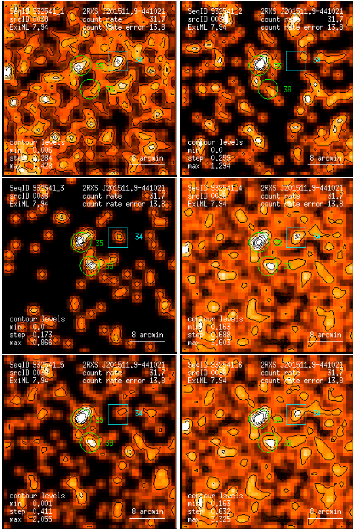
Figure 38: RASS 932541: detection 0038: band rate images, Gaussian filter: (1) PSPC channels 11 – 41, (2) 52 – 90, (3) 91 – 201, (4) 11 – 235, (5) 52 – 201, (6) 11 – 201. Broad band rates in counts/ks. Band rate contour levels in counts/ks/arcmin 2 .
